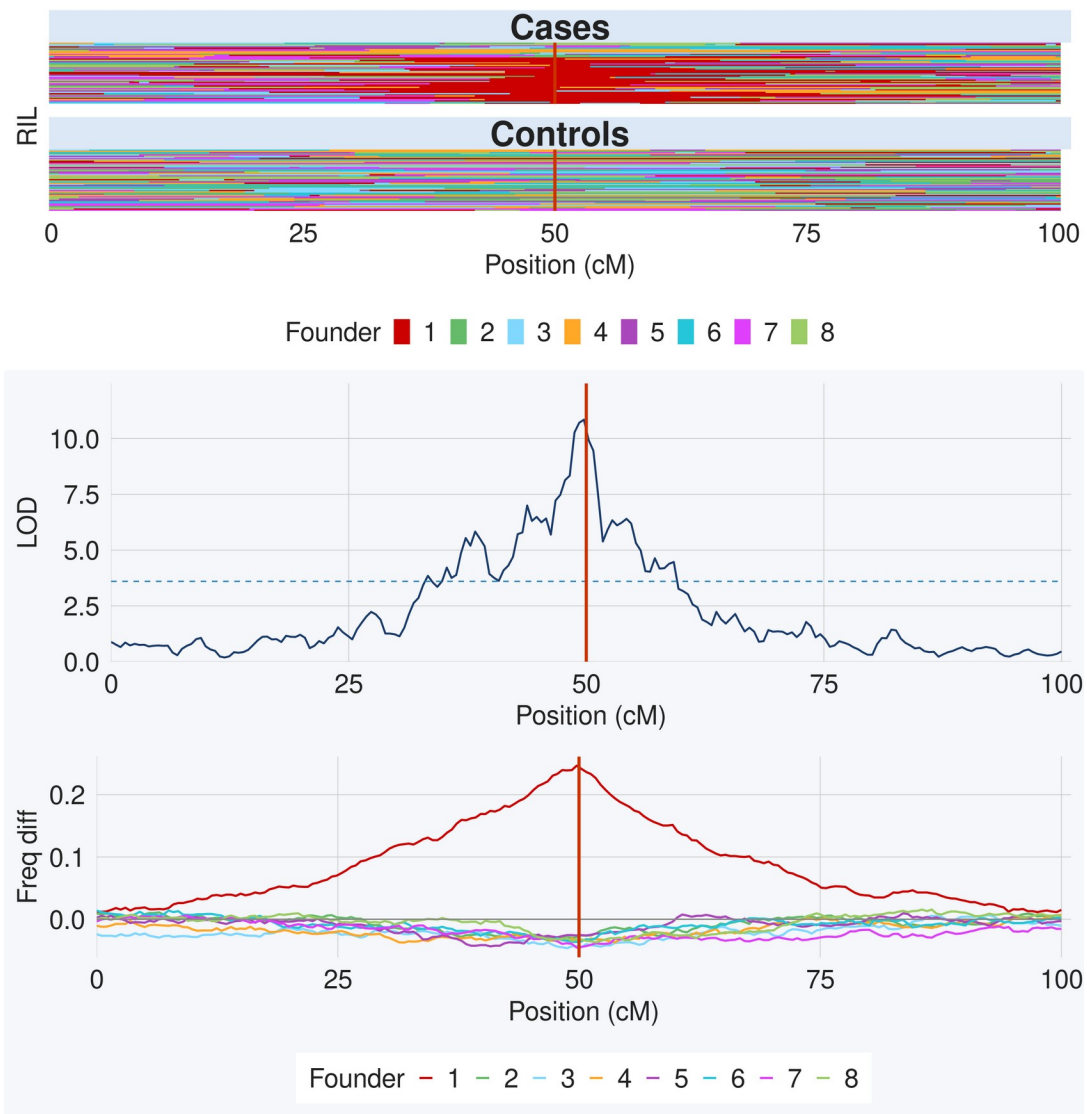
Figure 5. DSPR/BSA, 1 replicate × pool size 2,000 (same 6,000-individual total budget). 1 QTL architecture.
