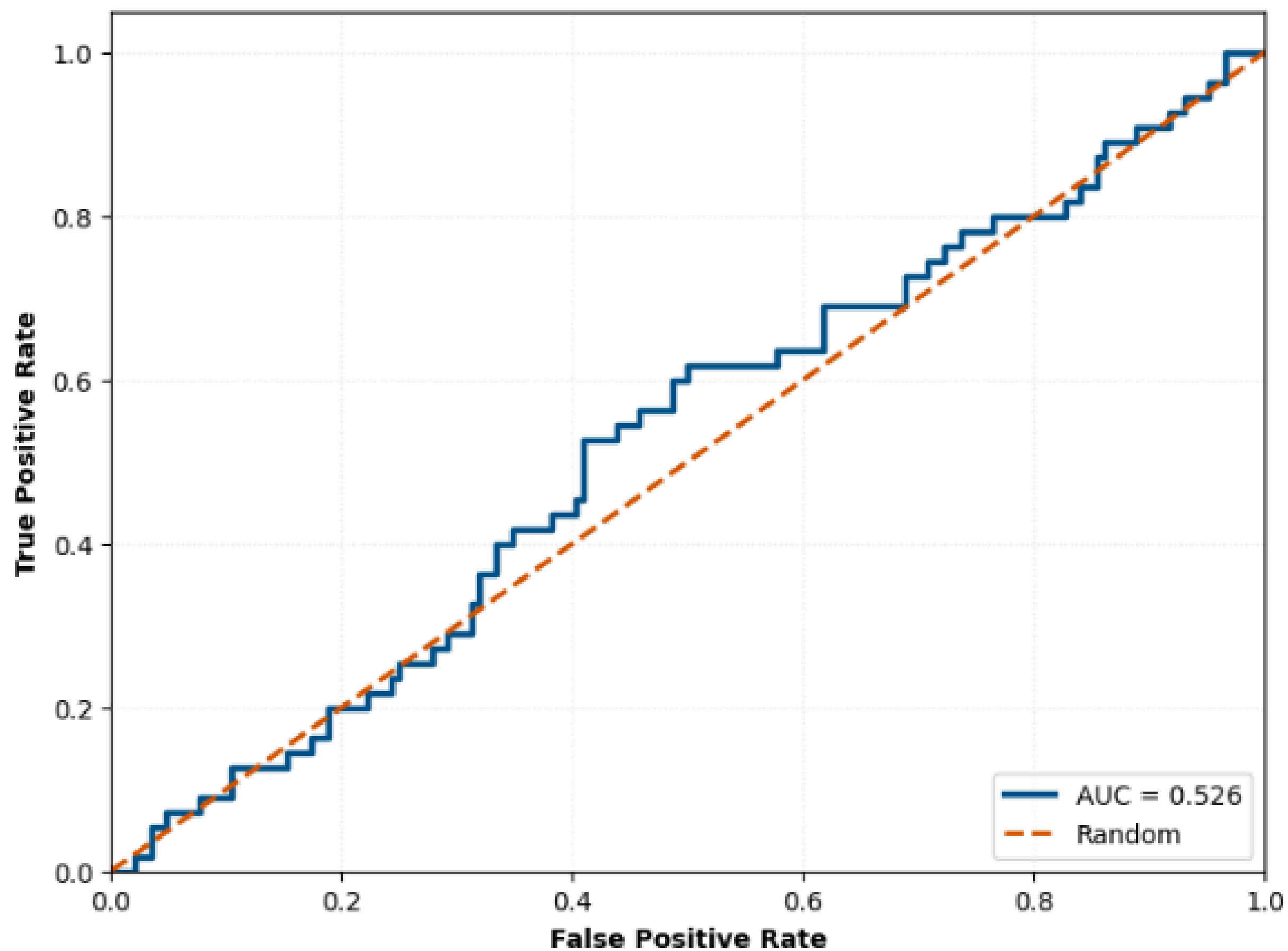
MobileNetV2 - ROC Curve
