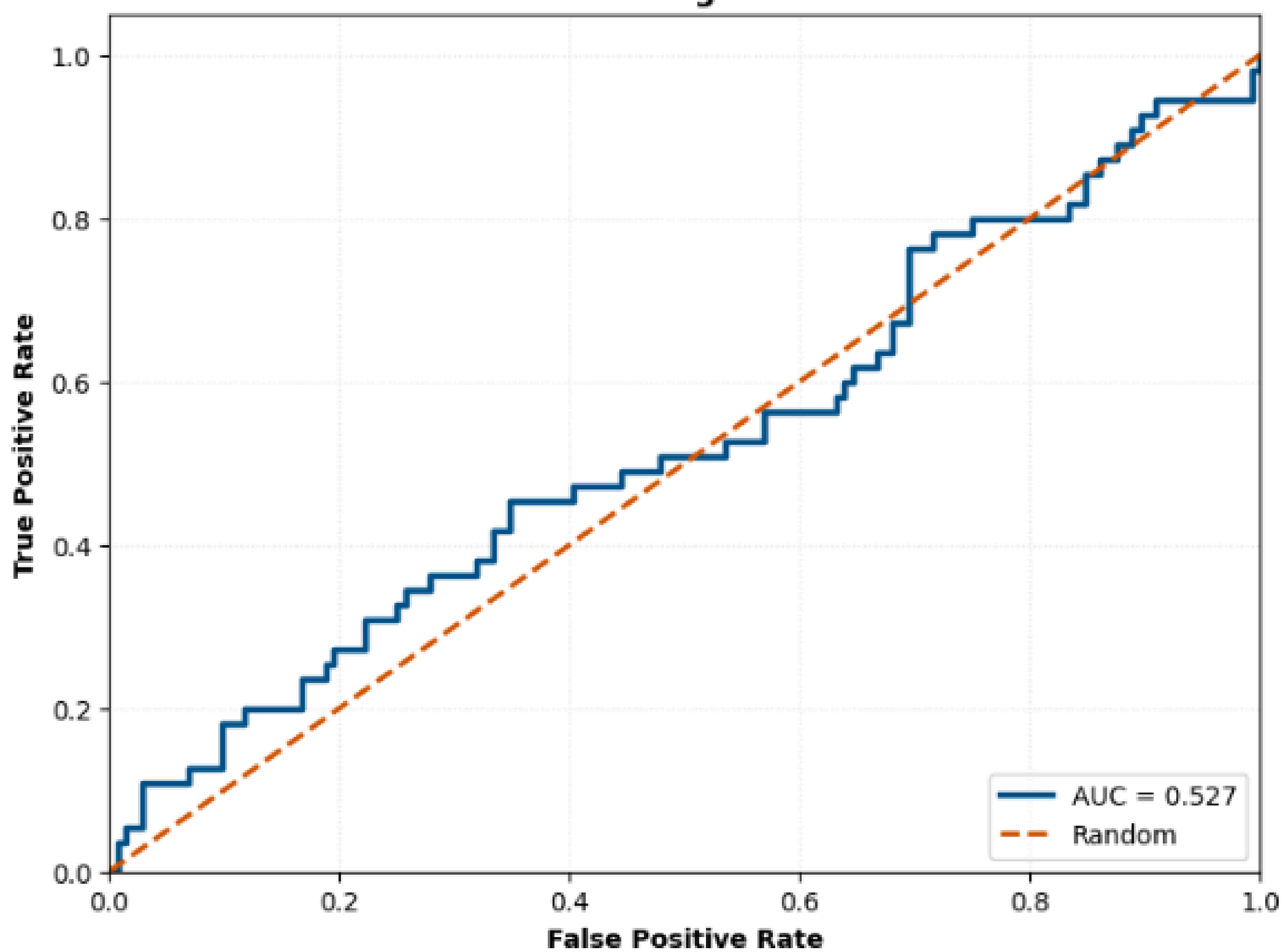
MobileNetV3Large - ROC Curve
