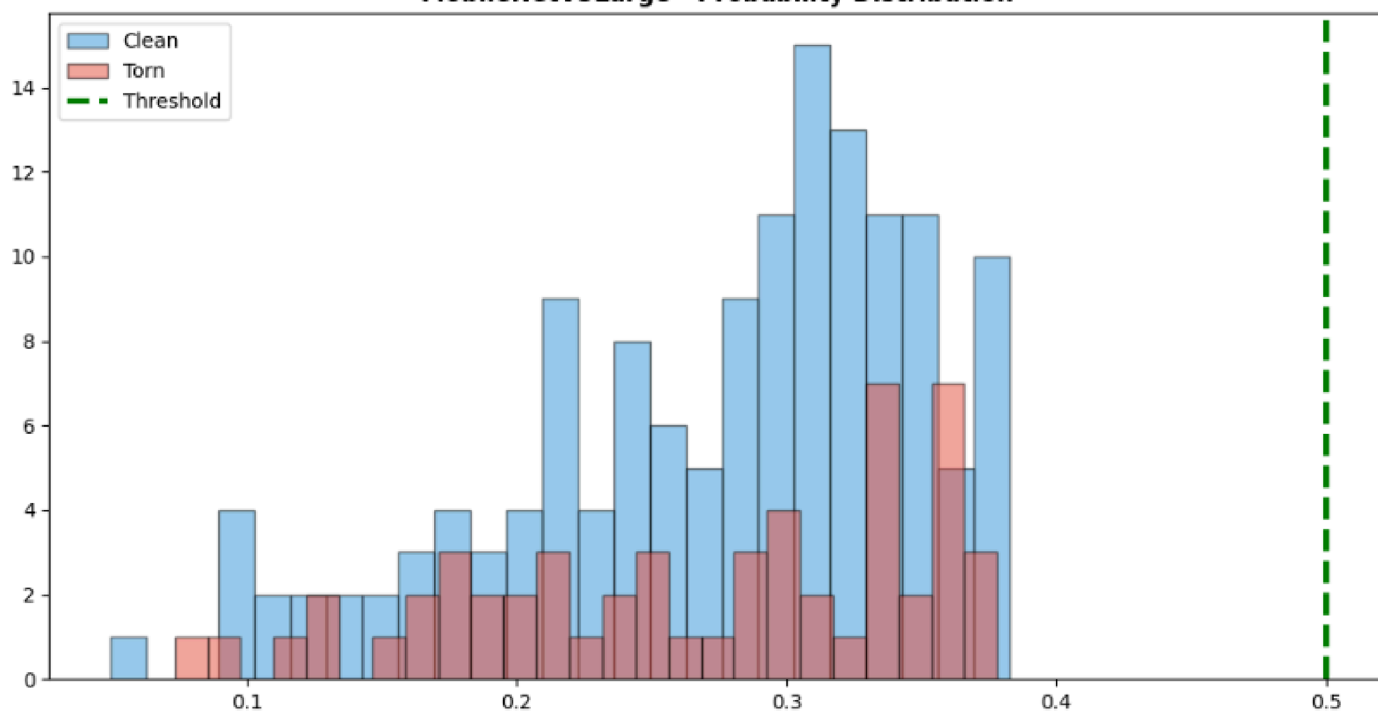
MobileNetV3Large - Probability Distribution
