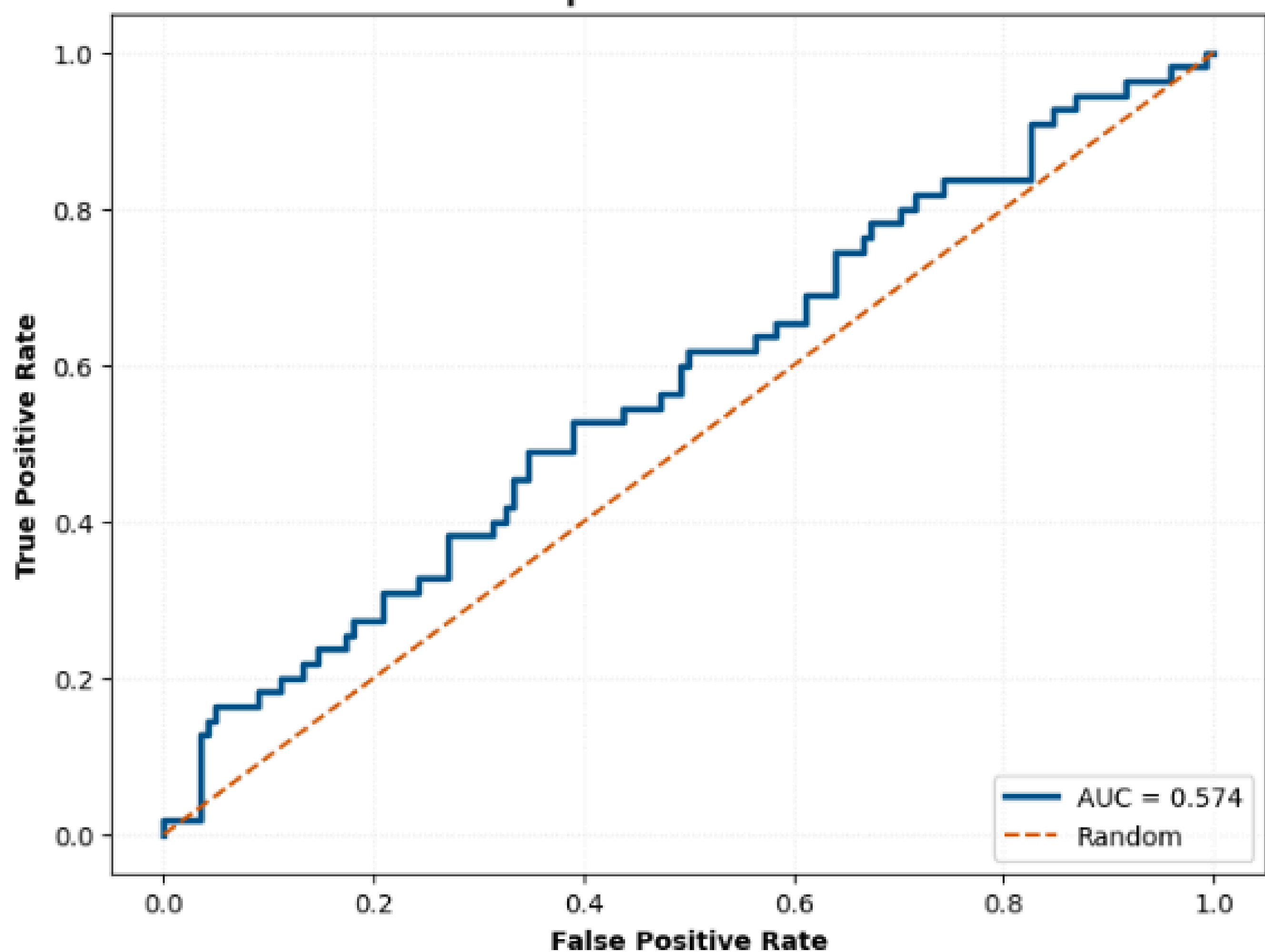
Xception - ROC Curve
