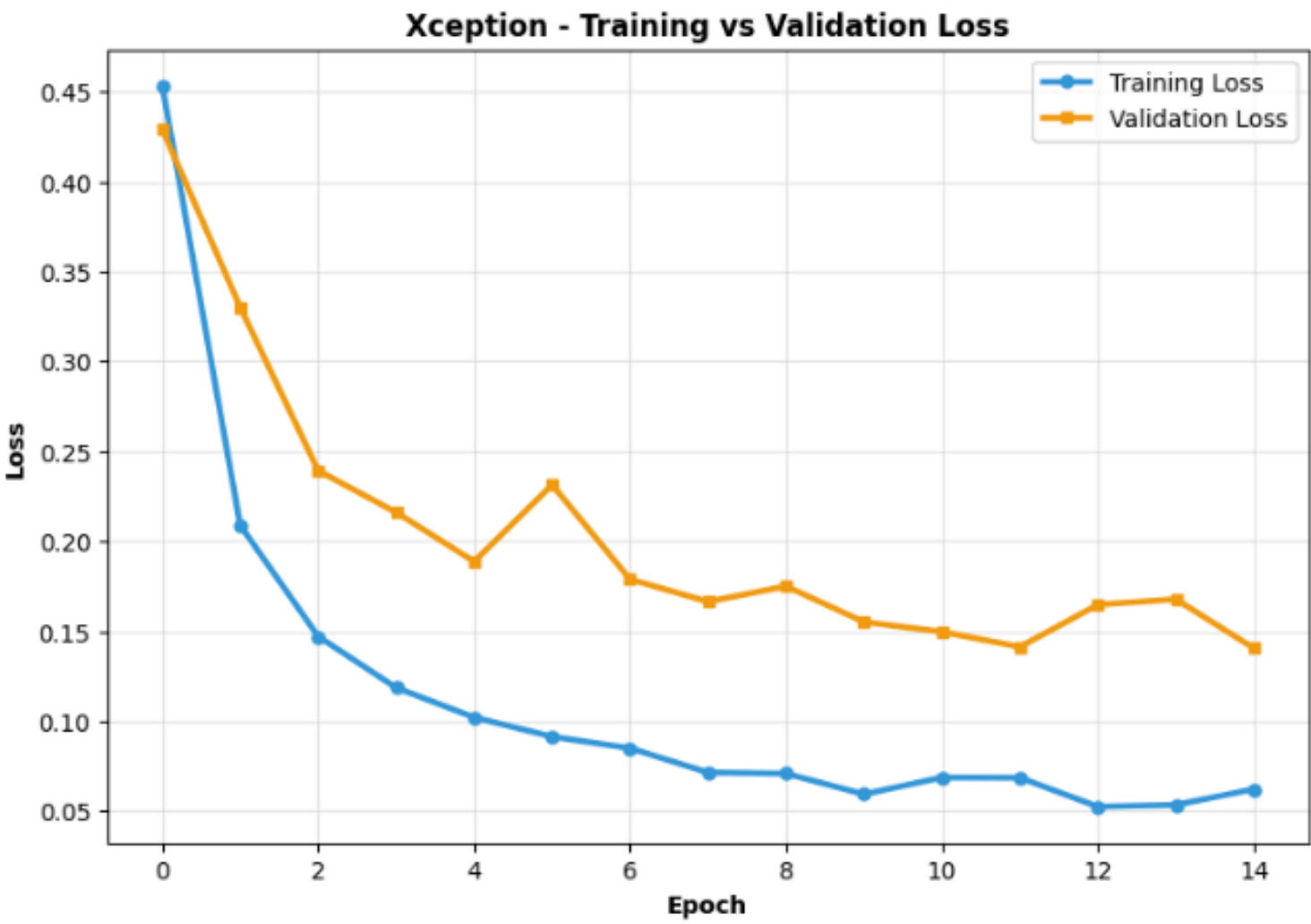
Xception - Comprehensive Error Analysis
