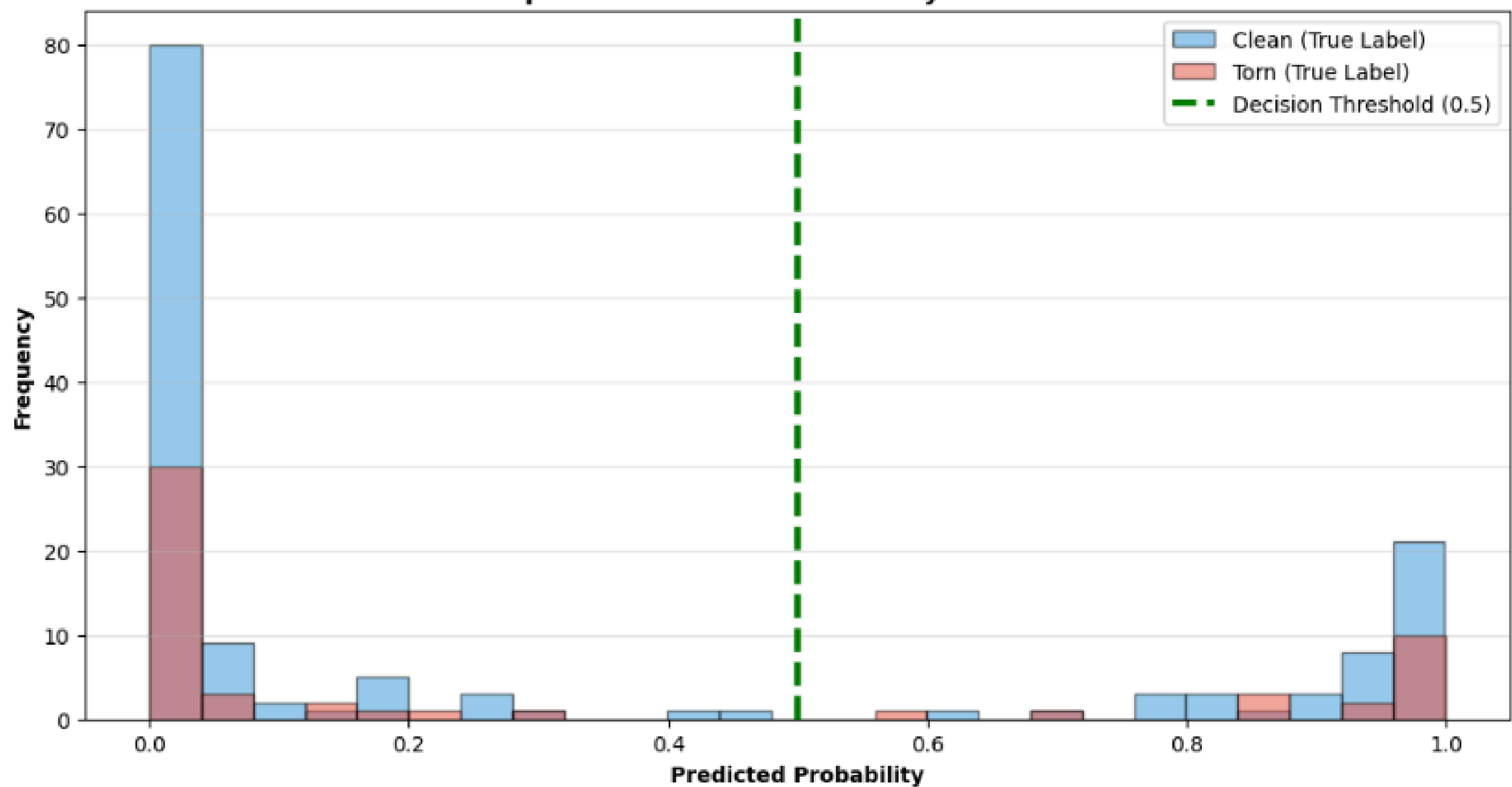
Xception - Prediction Probability Distribution
