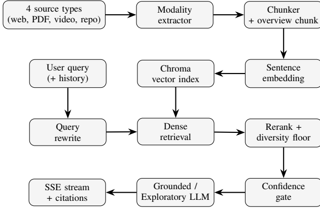
Fig. 1. SAGE end-to-end architecture: a shared ingest-chunk-embed-index contract across four source types feeds a single retrieve-rerank-gate-generate query pipeline.
