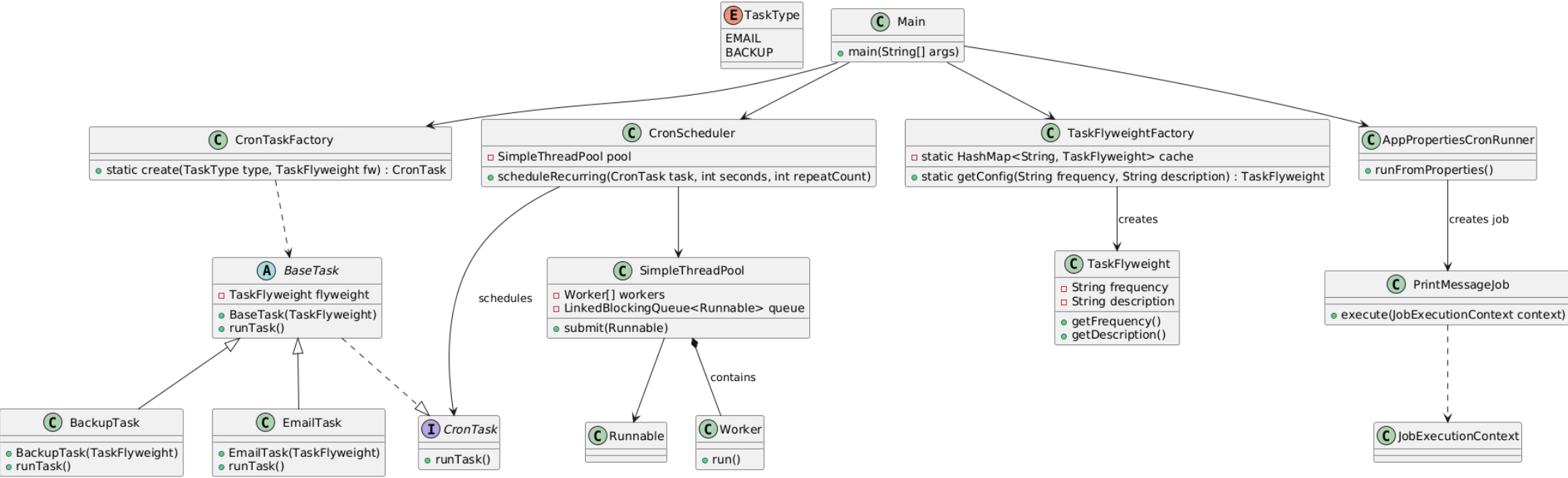
Cron Job Simulator - Class Diagram (Flyweight + Factory + ThreadPool + Properties Cron)
