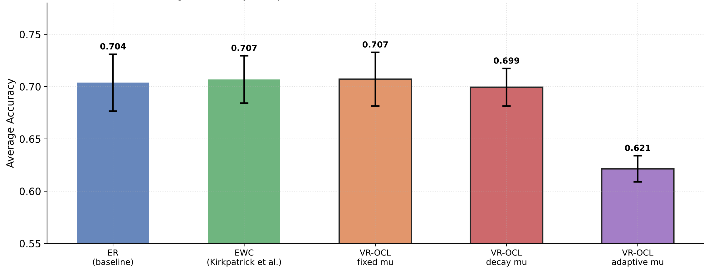
Average Accuracy — Split CIFAR-10 (mem=500, \mu=0.0005 for VR methods)
