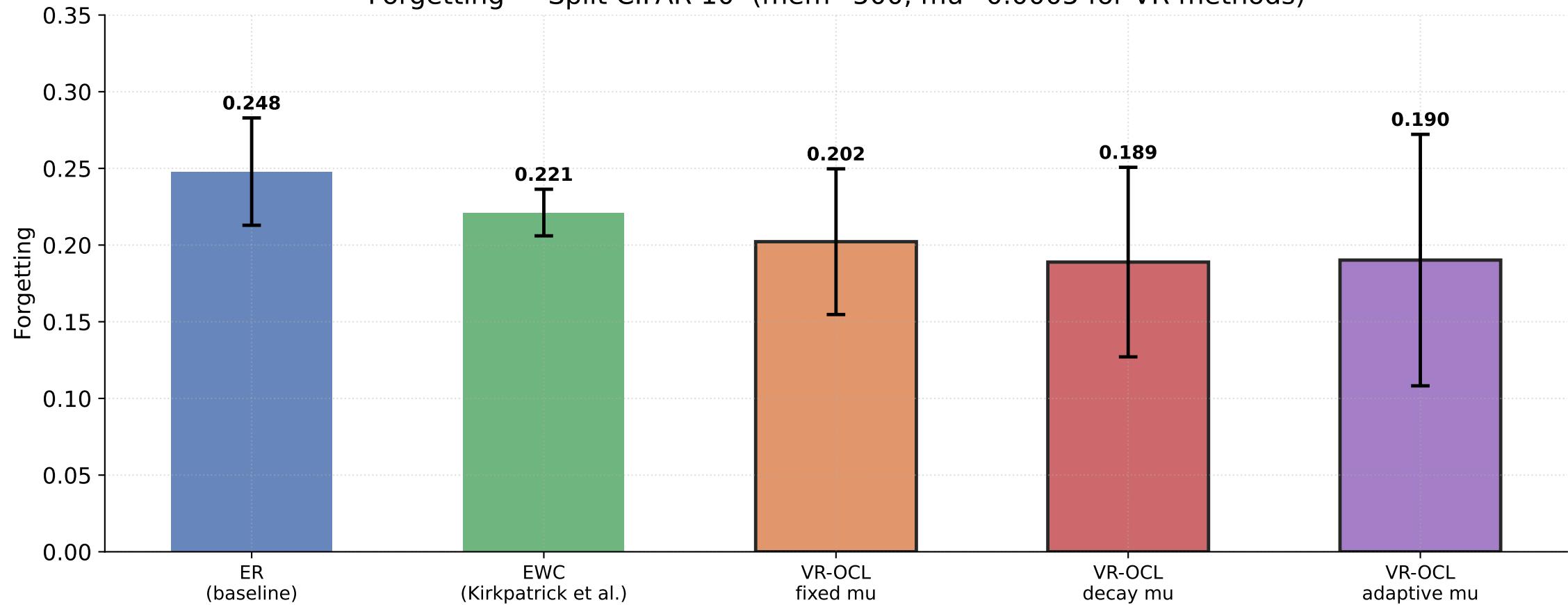
Forgetting — Split CIFAR-10 (mem=500, \mu=0.0005 for VR methods)
