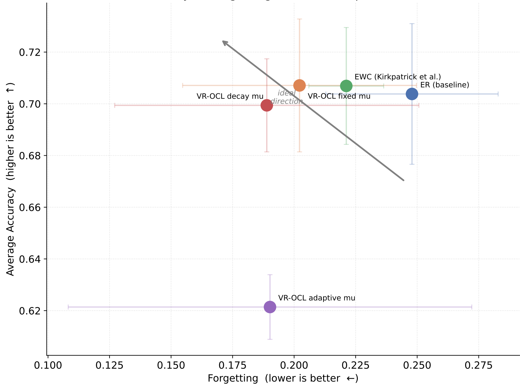
Accuracy vs Forgetting Trade-off — Split CIFAR-10
