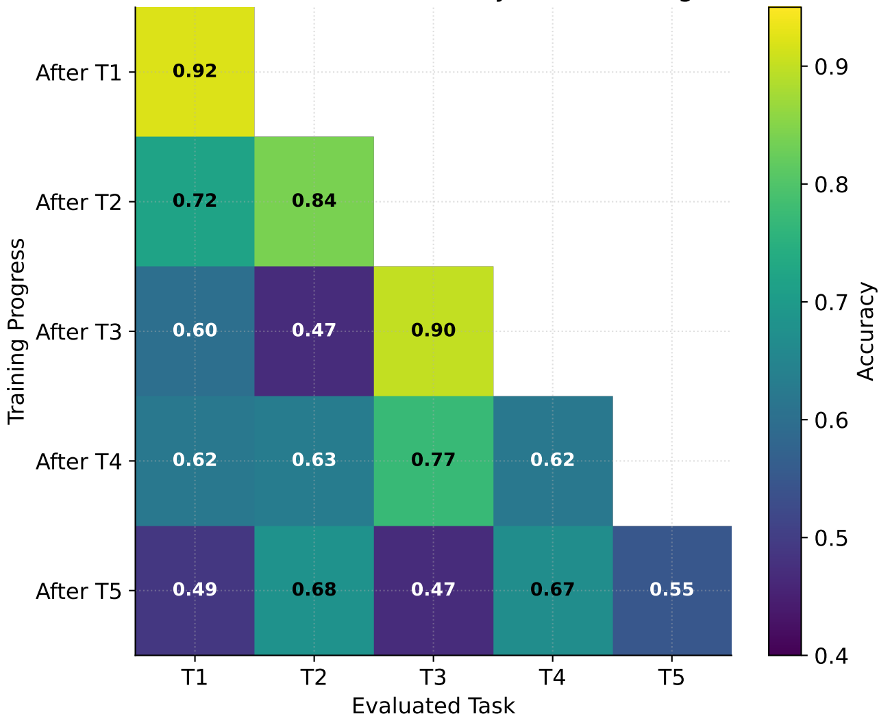
EWC — Per-Task Accuracy Over Training
