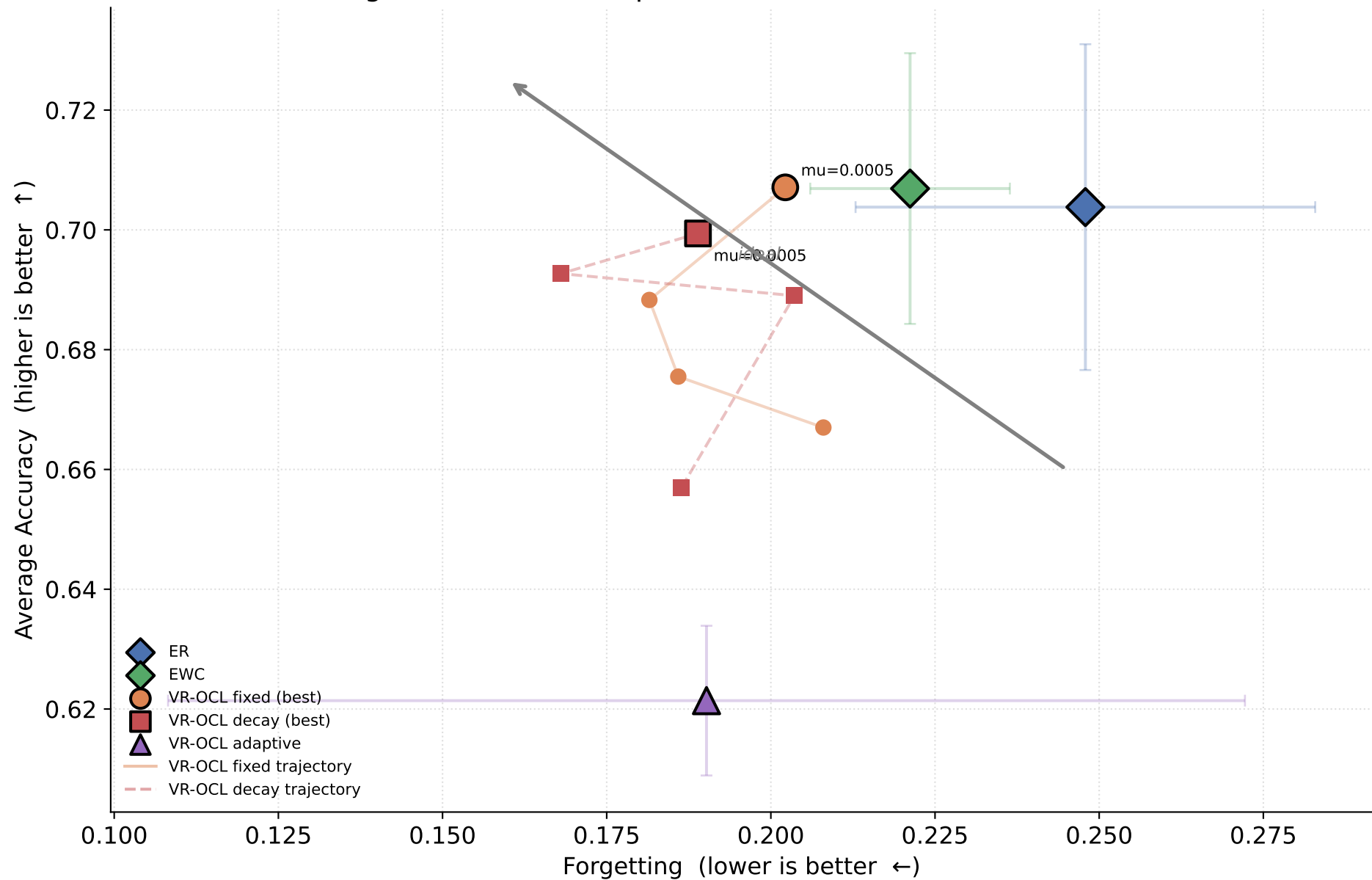
Full Stability-Plasticity Tradeoff — All VR-OCL Variants (Large markers = best per method, small = other \mu values)
