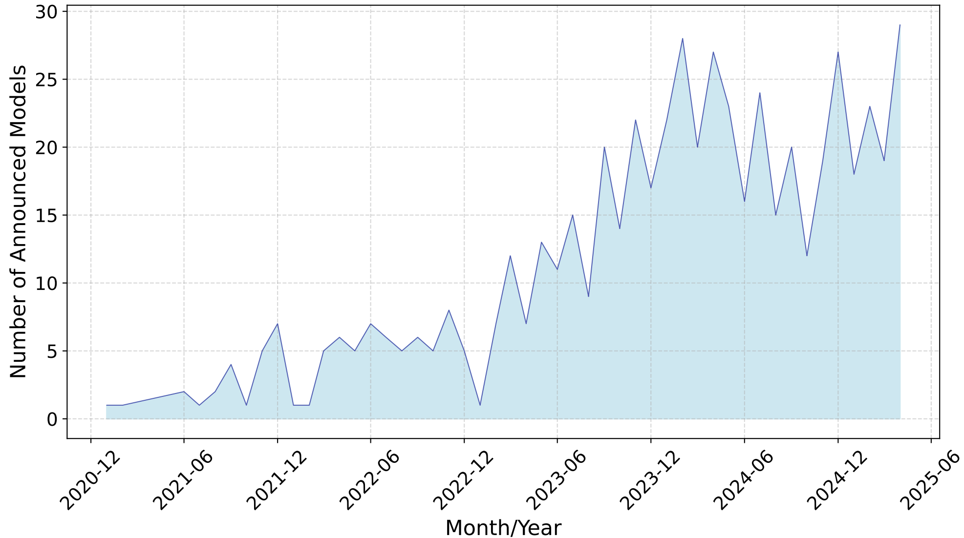
Number of LLM Releases Over Time
