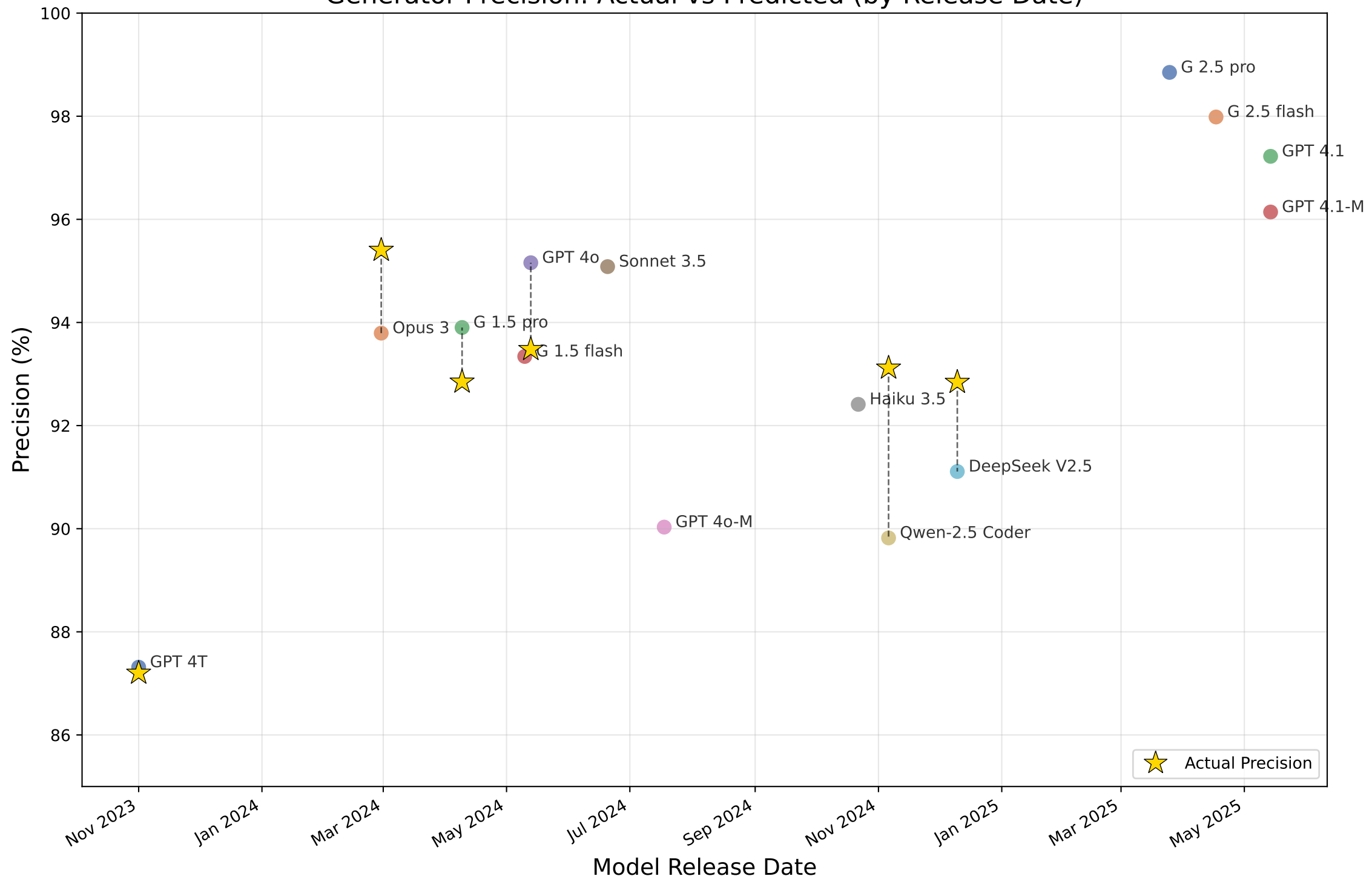
Generator Precision: Actual vs Predicted (by Release Date)
