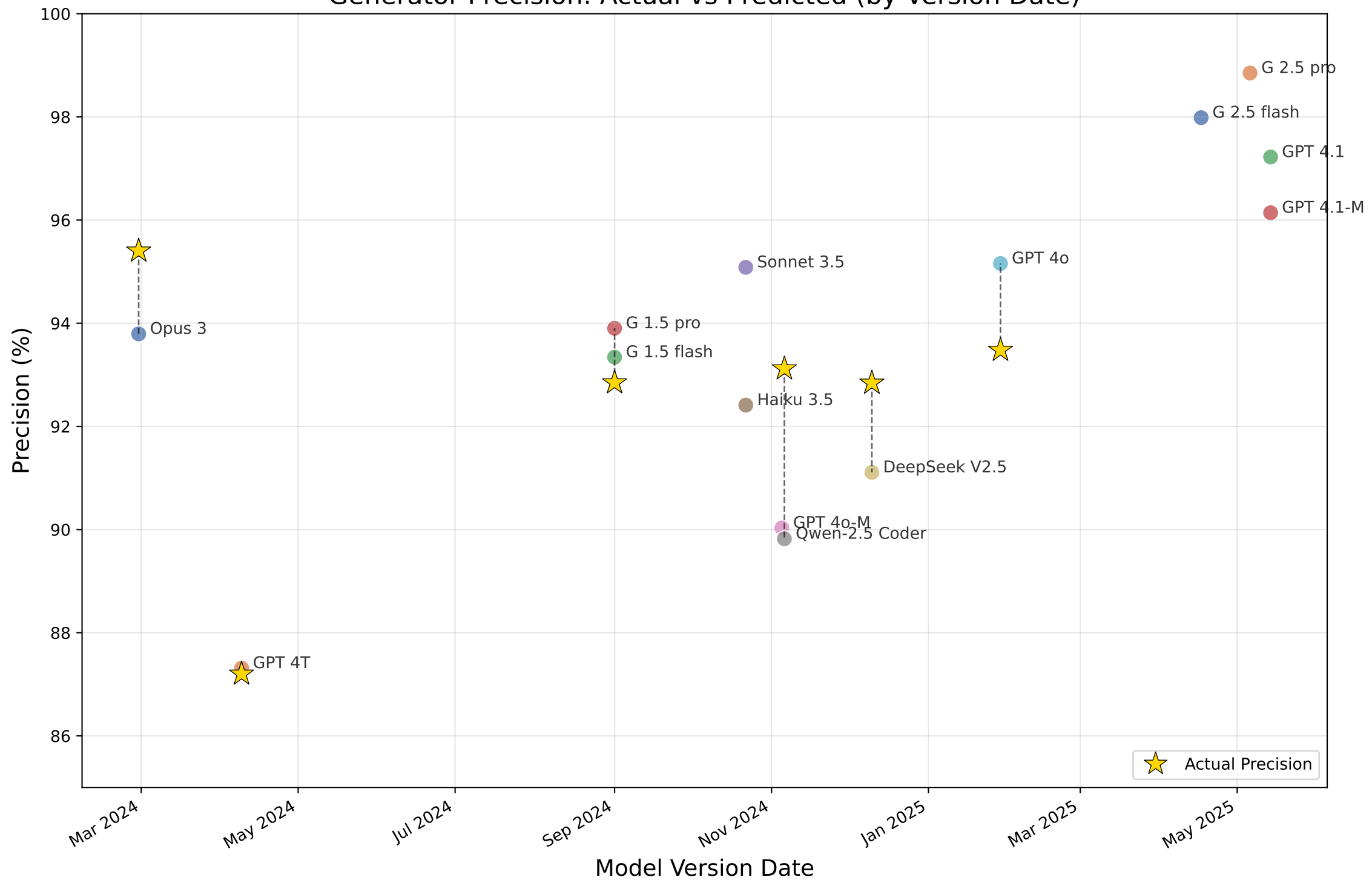
Generator Precision: Actual vs Predicted (by Version Date)
