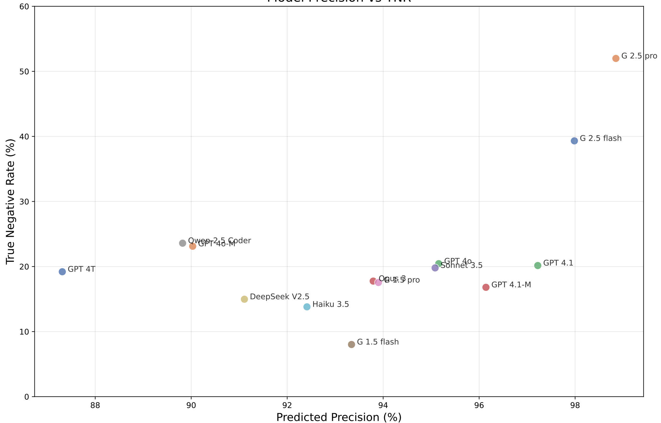
Model Precision vs TNR
