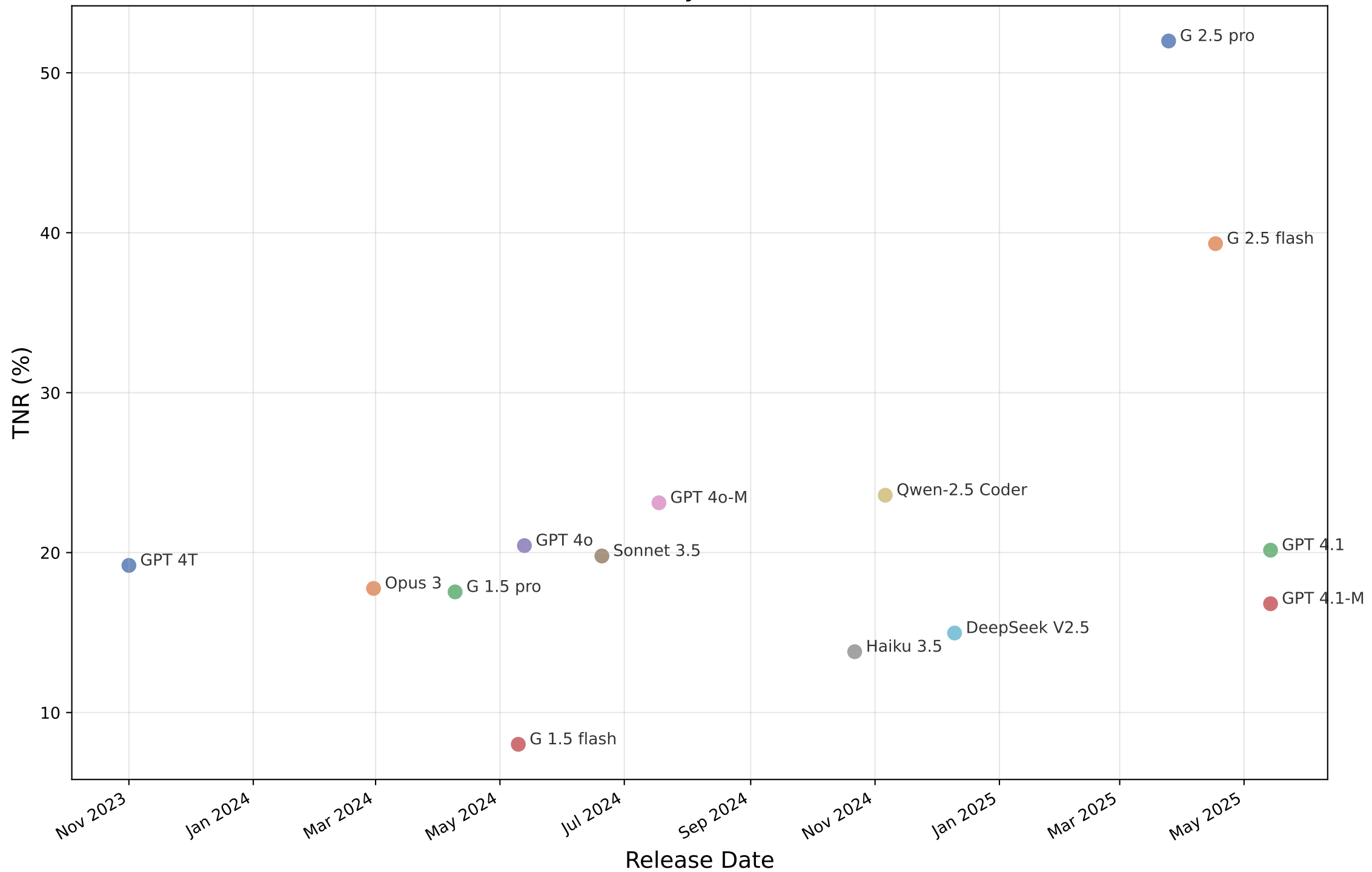
Model TNR by Release Date
