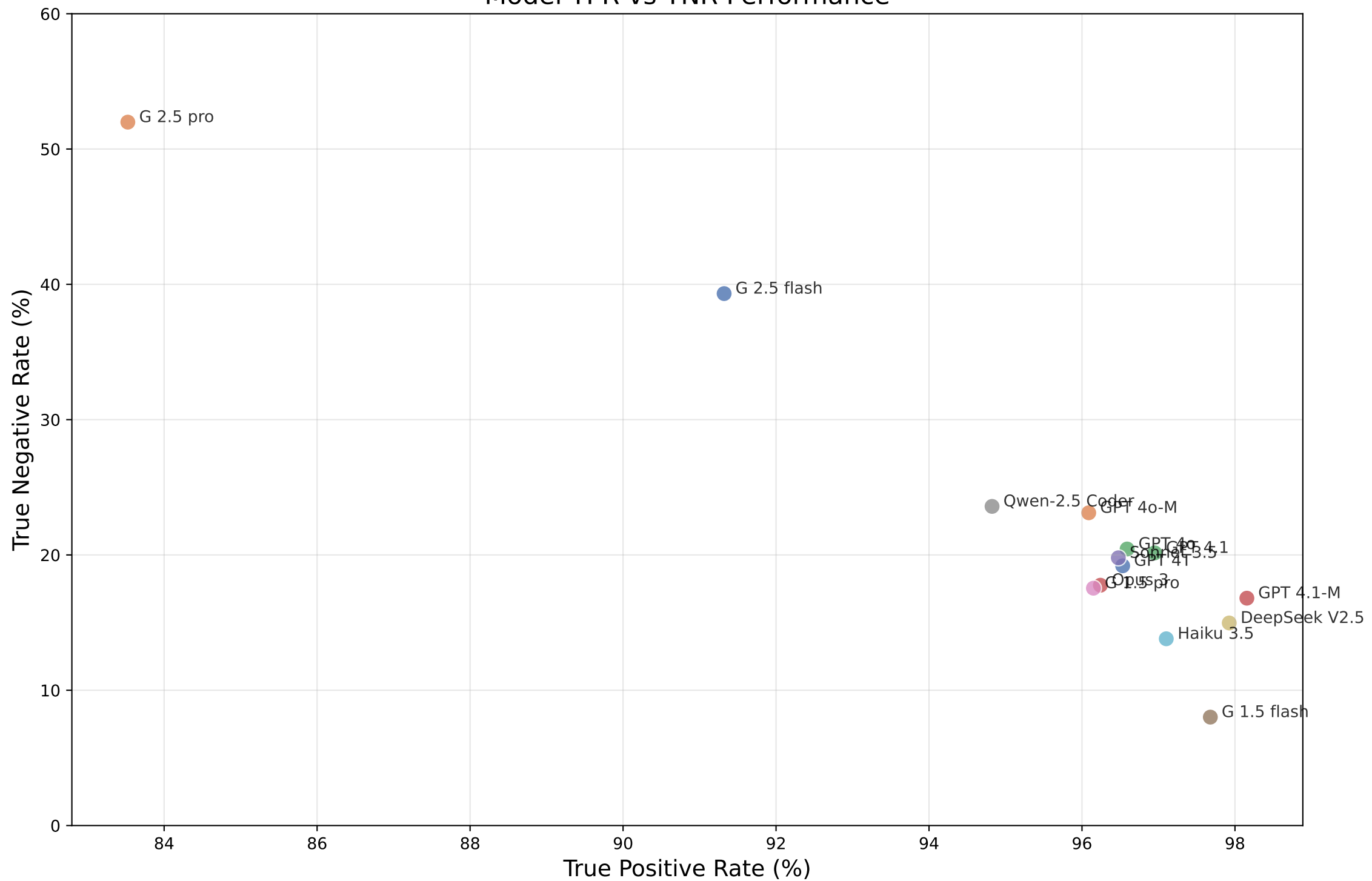
Model TPR vs TNR Performance
