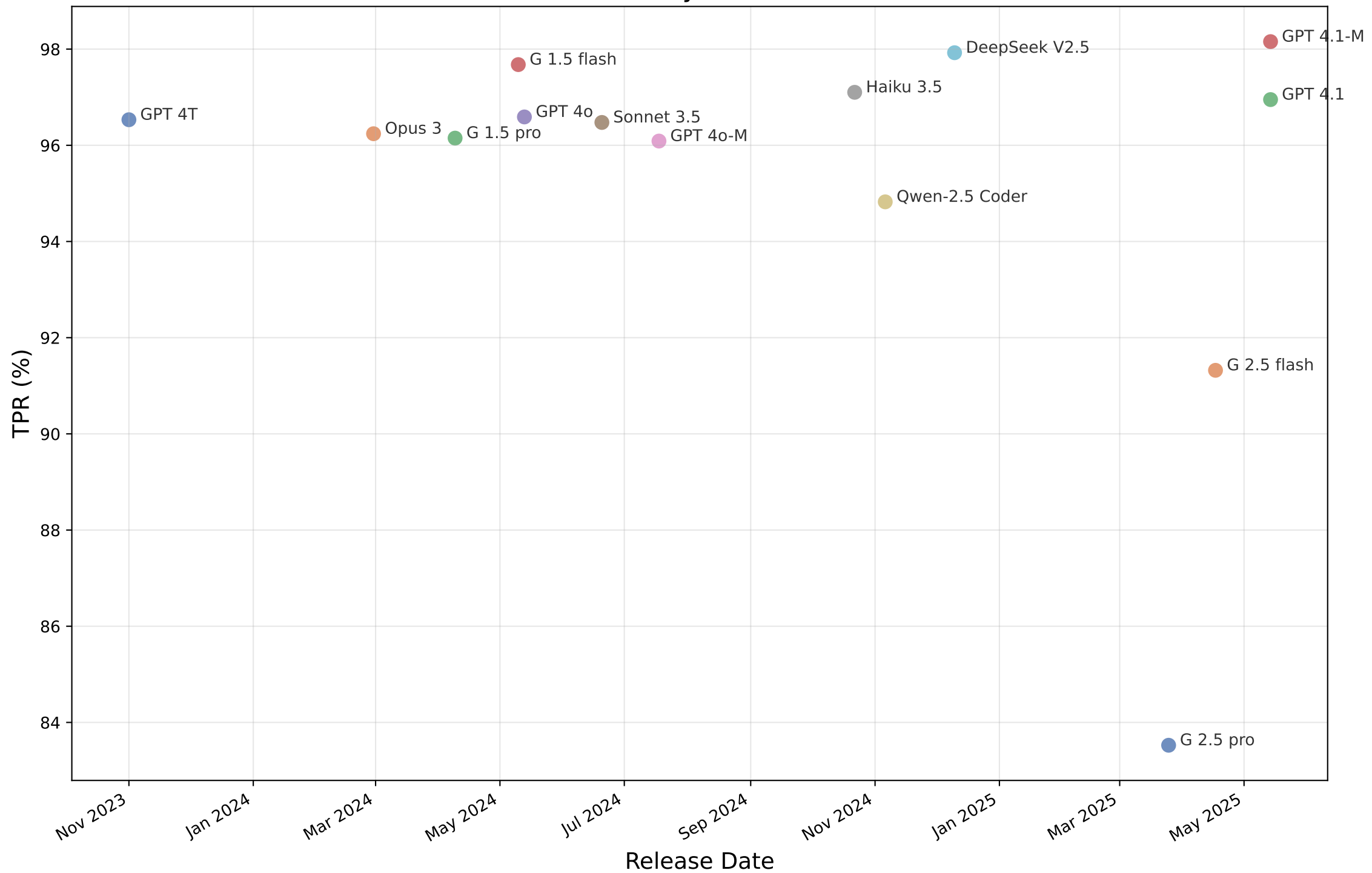
Model TPR by Release Date
