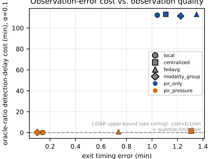
Observation-error cost vs. observation quality
