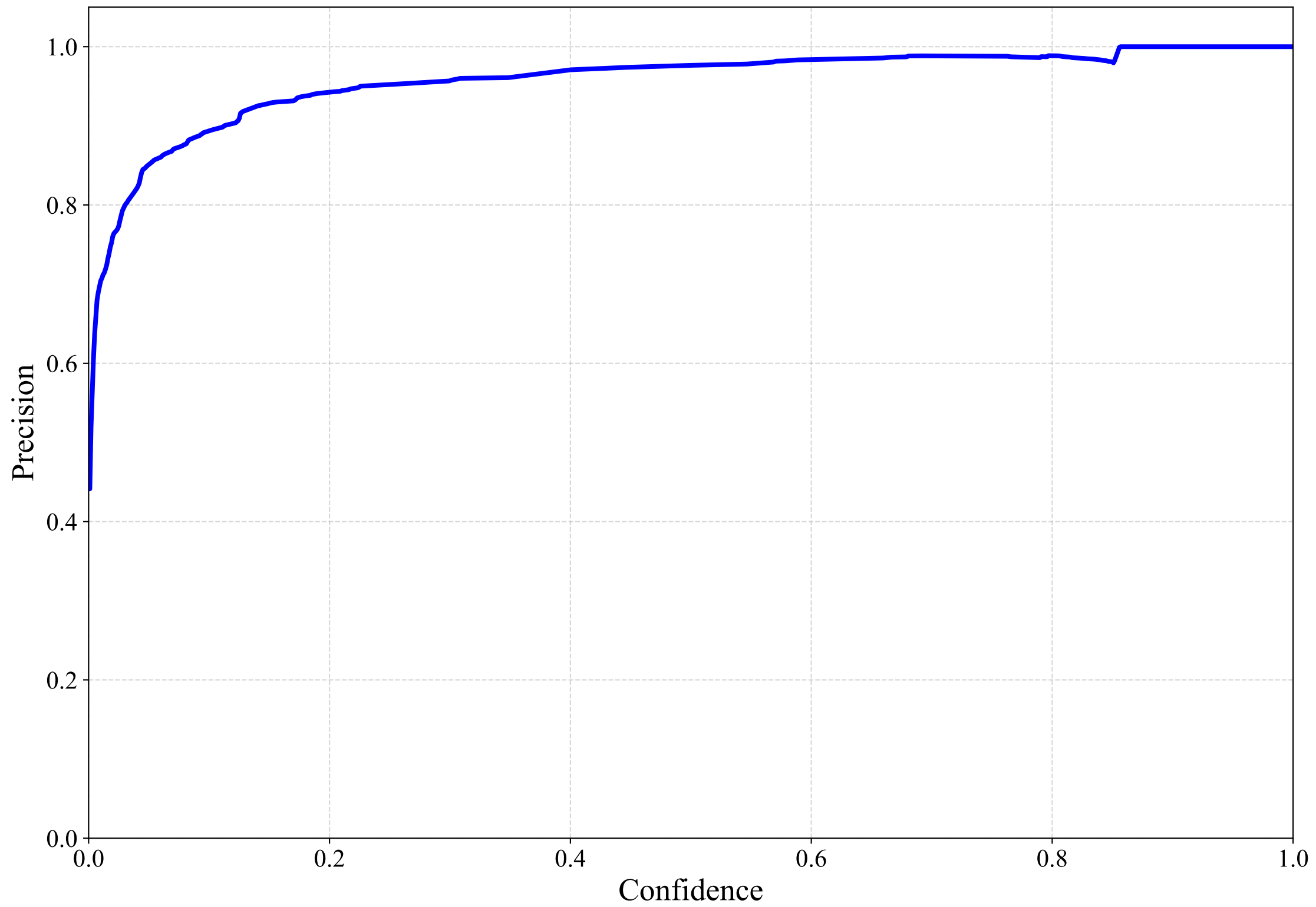
Precision-Confidence Curve
