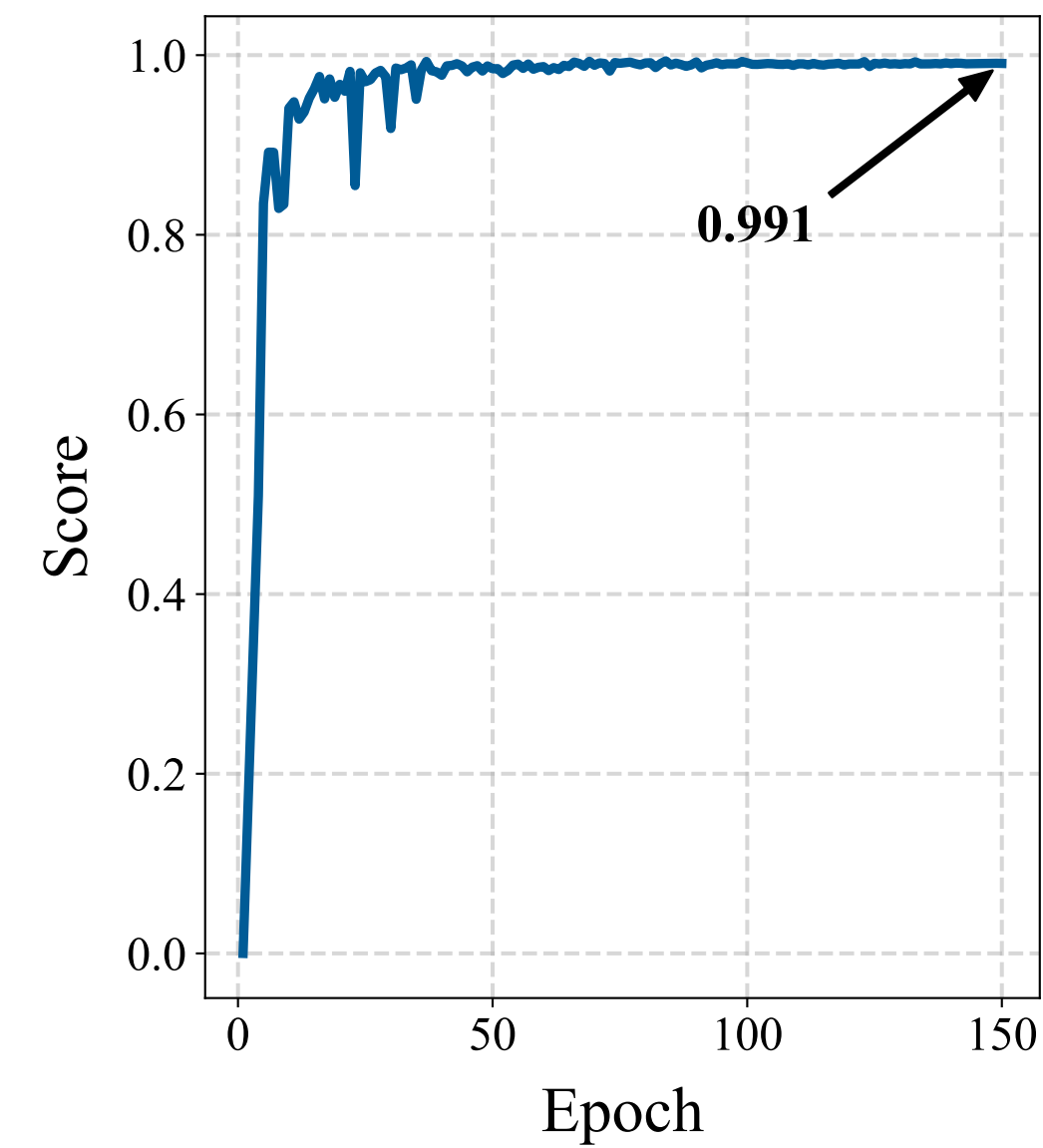
mAP @ 0.5
