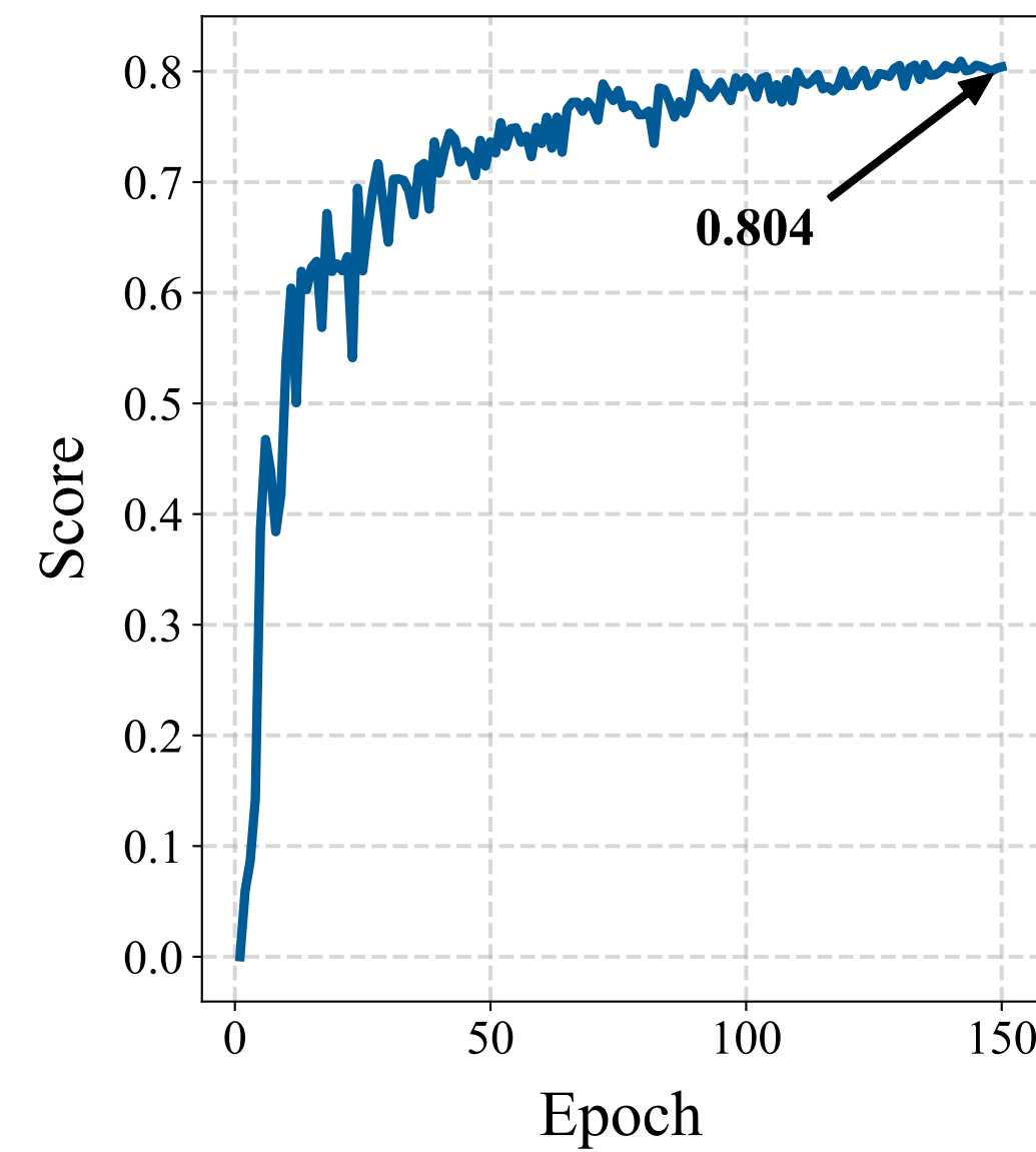
mAP @ 0.5:0.95
