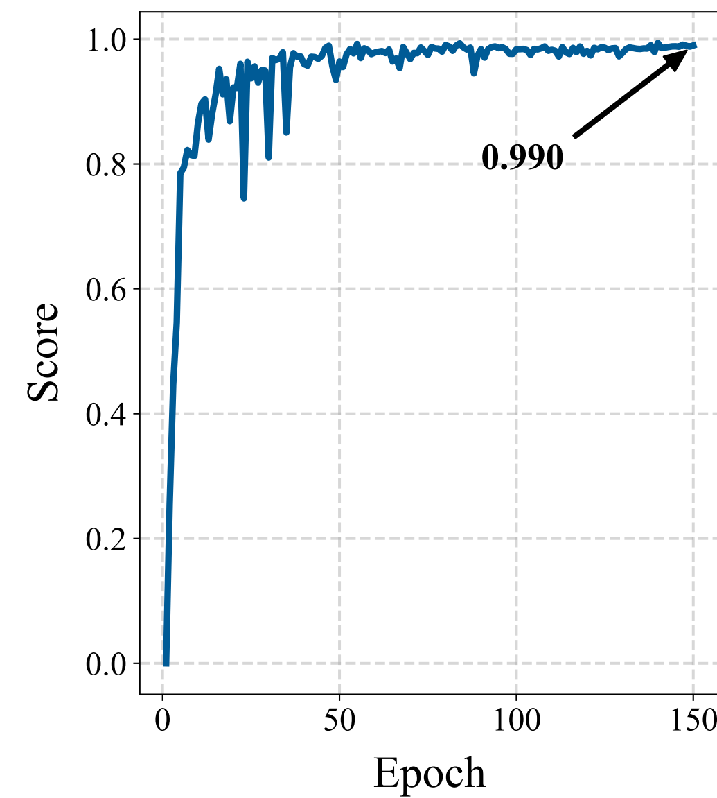
Recall (B)
