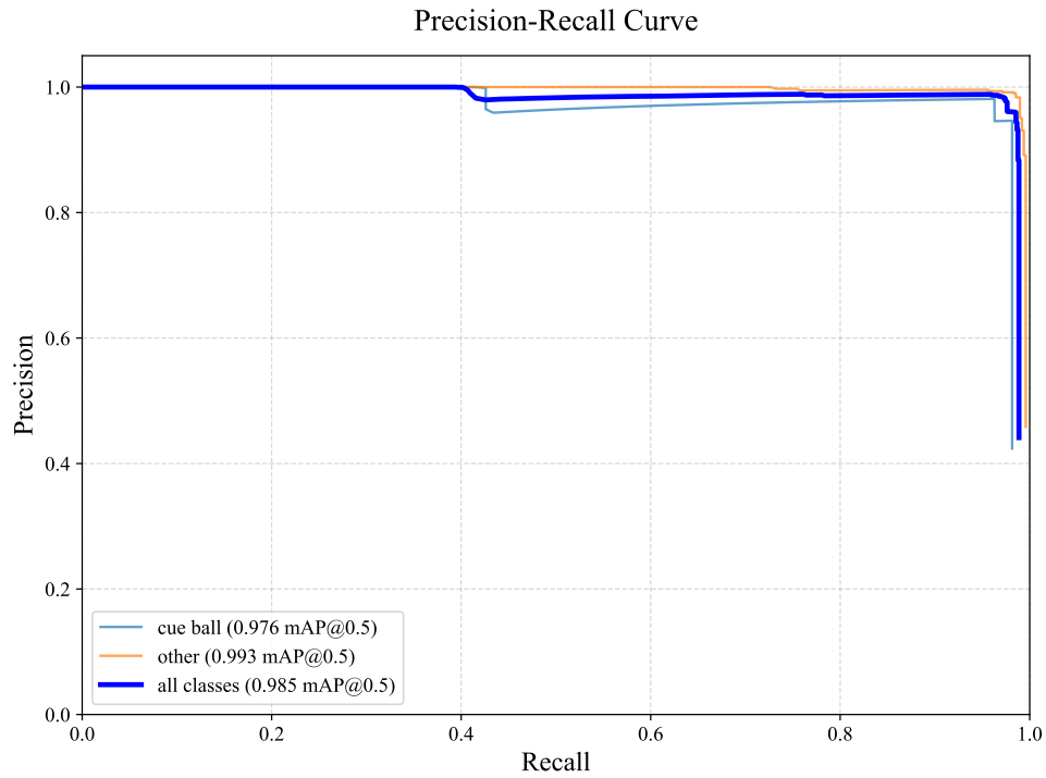
Figure 6.2: Precision-Recall Curve showing mAP@0.5 of 0.985 for the Ball Detection model.
