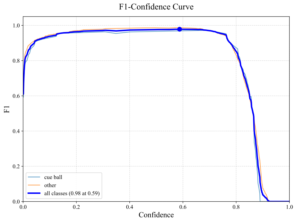
Figure 6.3: F1-Confidence Curve indicating the optimal confidence threshold of 0.59.
