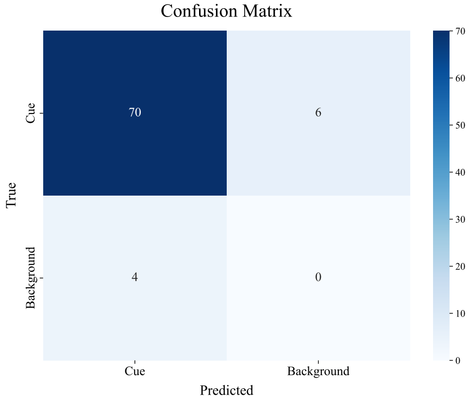
Figure 6.8: Confusion Matrix for Cue Detection, showing 70 correct detections against 6 false negatives (background).
