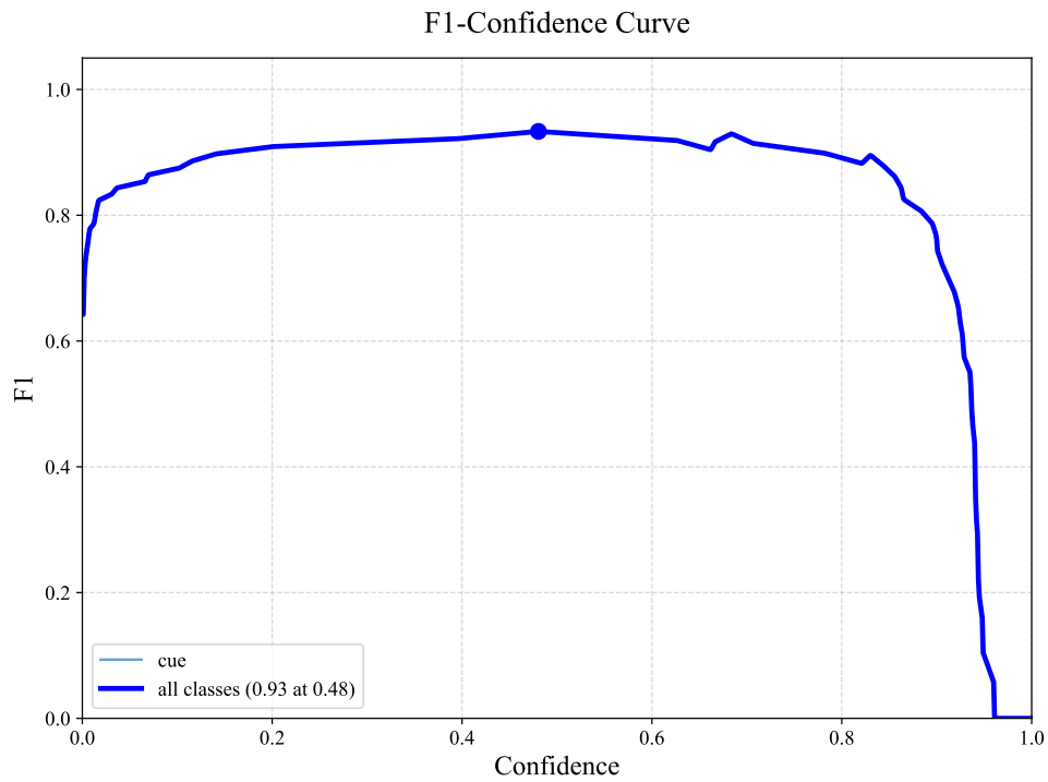
Figure 6.7: F1-Confidence Curve for the cue stick keypoints, peaking at 0.93.
