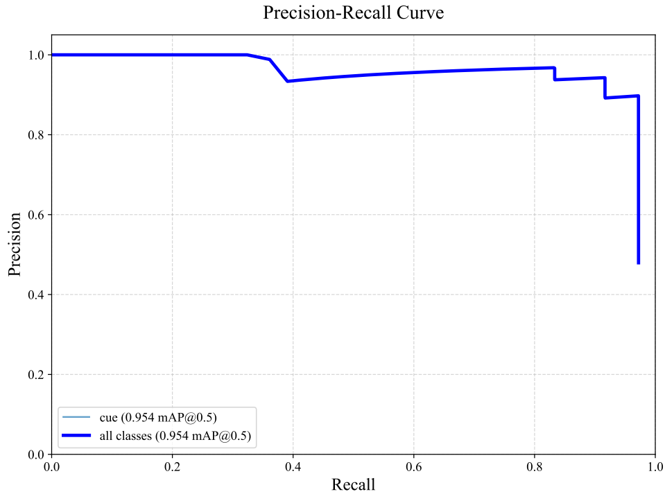
Figure 6.6: Precision-Recall Curve for Pose Estimation showing a high mAP@0.5 of 0.954.
