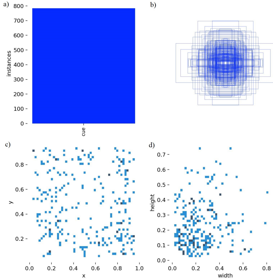
Figure 3.3: Analysis of the cue detection dataset: (a) Single-class distribution; (b) Bounding box density map; (c) Spatial distribution of cue centers; (d) Correlation of bounding box width and height.
