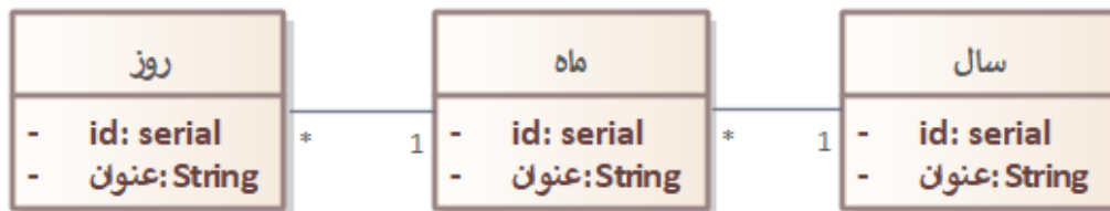
class Basic Class Diagram with Attributes
