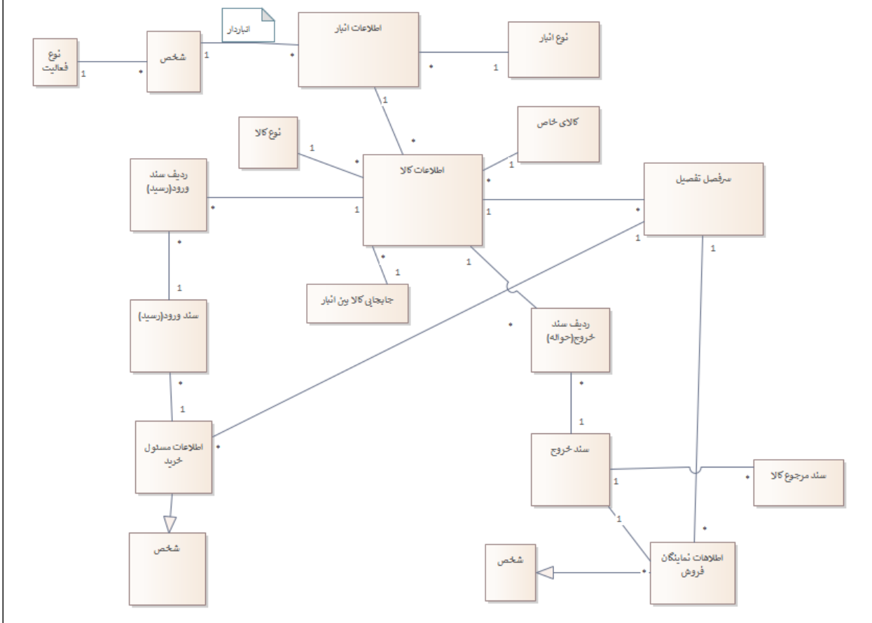
class Basic Class Diagram with Multiplicities
