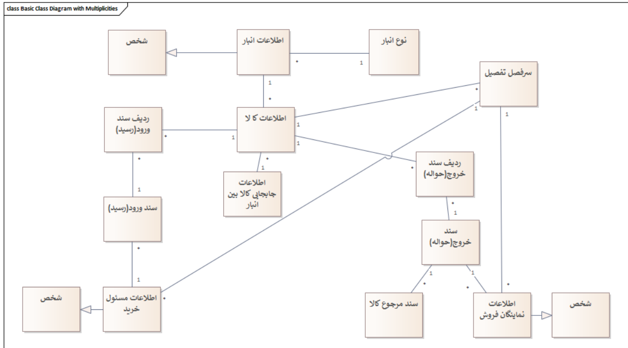
class Basic Class Diagram with Multiplicities
