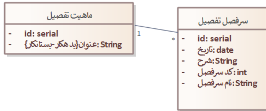
class Basic Class Diagram with Attributes
