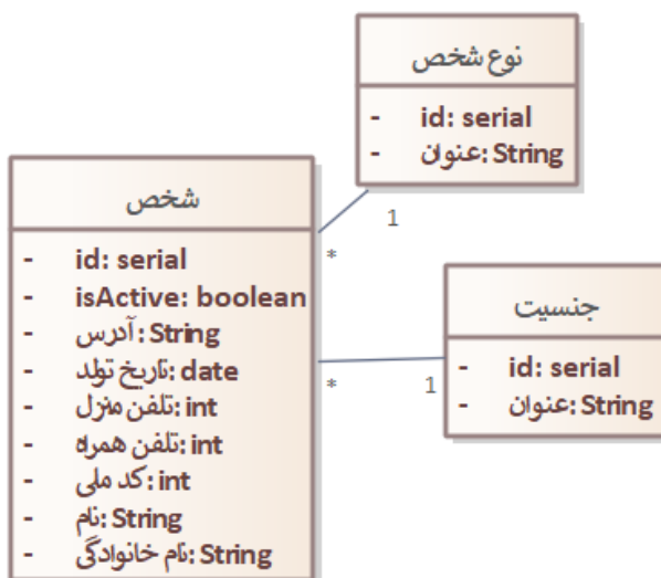
class Basic Class Diagram with Attributes
