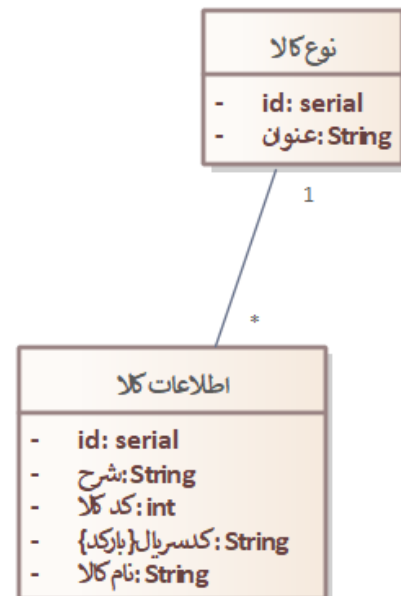
class Basic Class Diagram with Attributes
