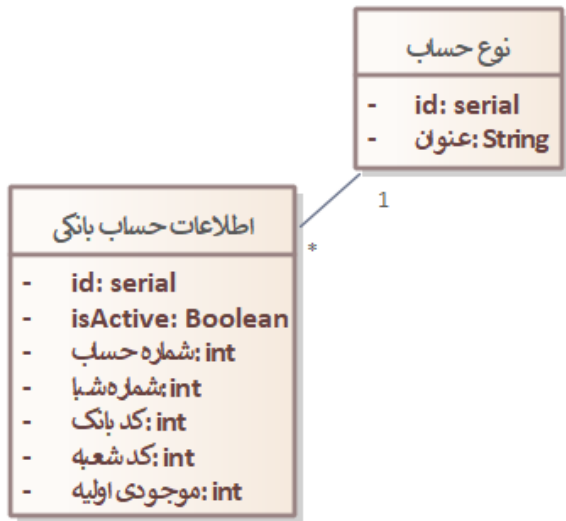
class Basic Class Diagram with Attributes
