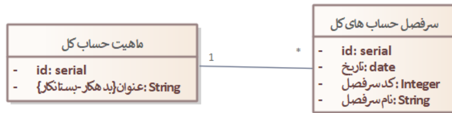
class Basic Class Diagram with Attributes
