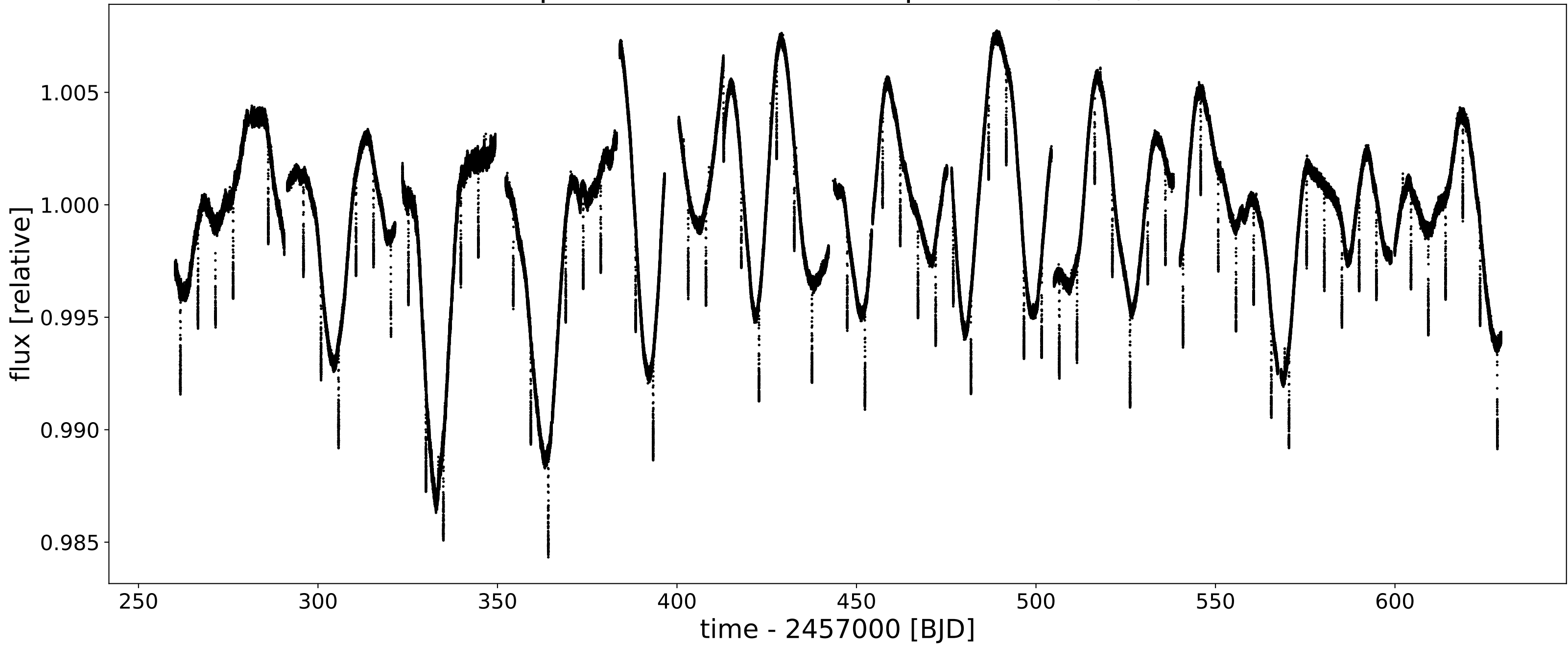
Kepler data for HAT-P-11 quarters 3, 4, 5, 6
