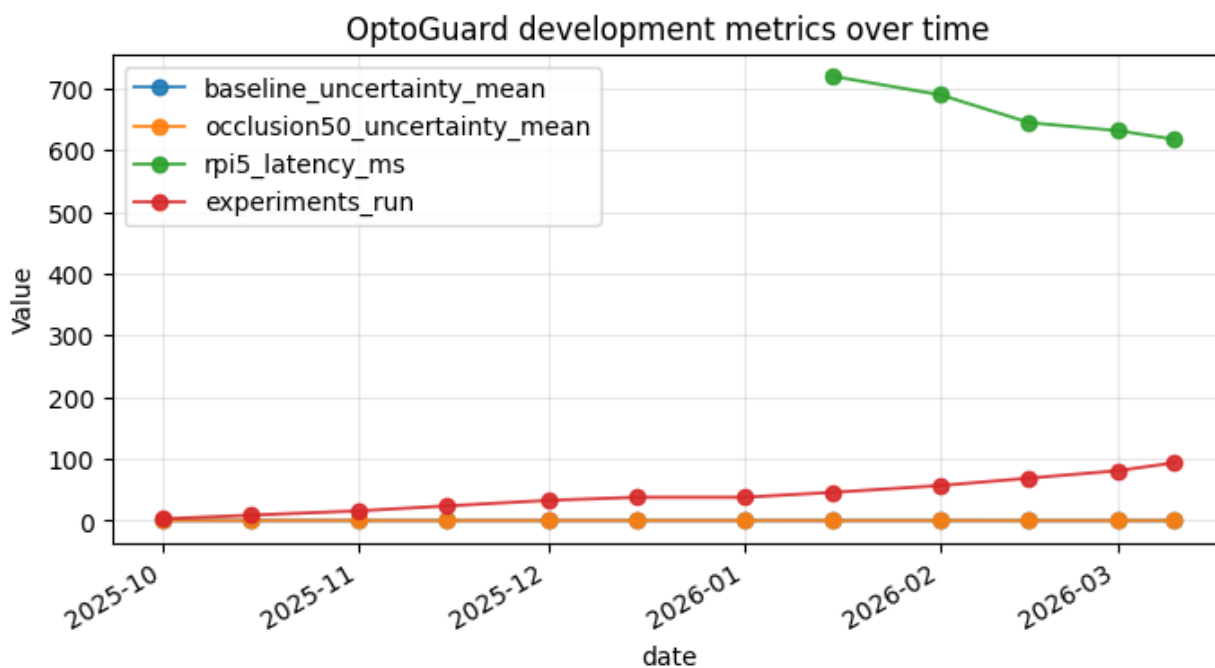
Figure 4. Development timeline (Oct 2025–Mar 2026)
