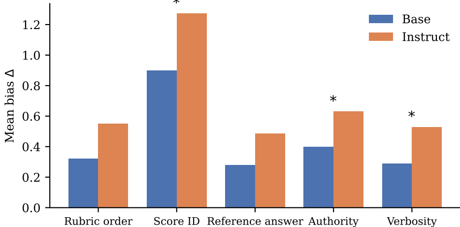
Scoring bias, base vs instruct ( n = 13 families)
