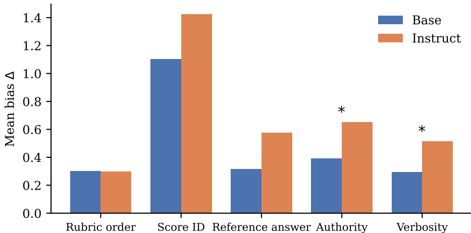
Scoring bias, base vs instruct ( n = 9 families)
