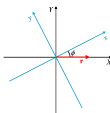
Figure 5.2: Diagram for 2D coordinate rotation. Black is lab frame, blue is molecule frame, and red is a vector that just happens to be aligned with the lab frame.
