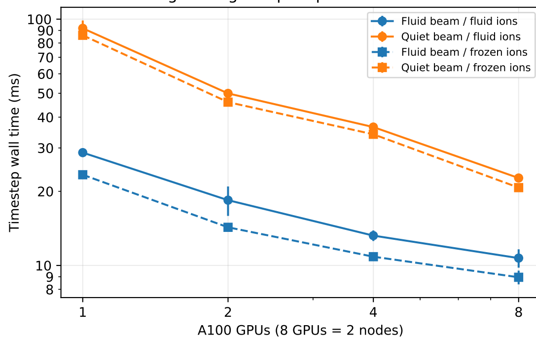
Strong scaling: coupled production and MCC
