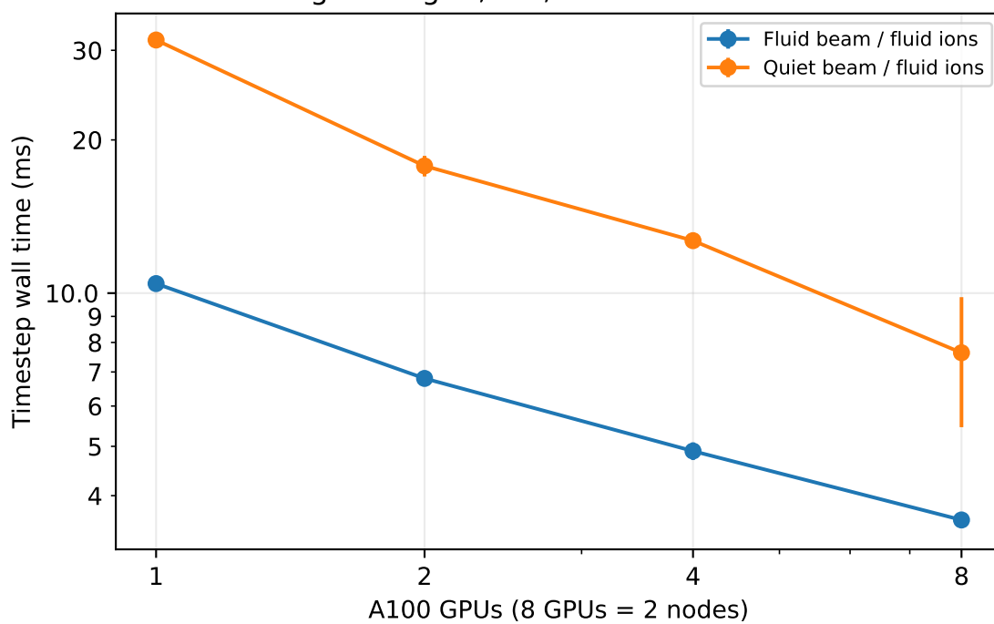
Strong scaling: 1,048,576 identical electrons
