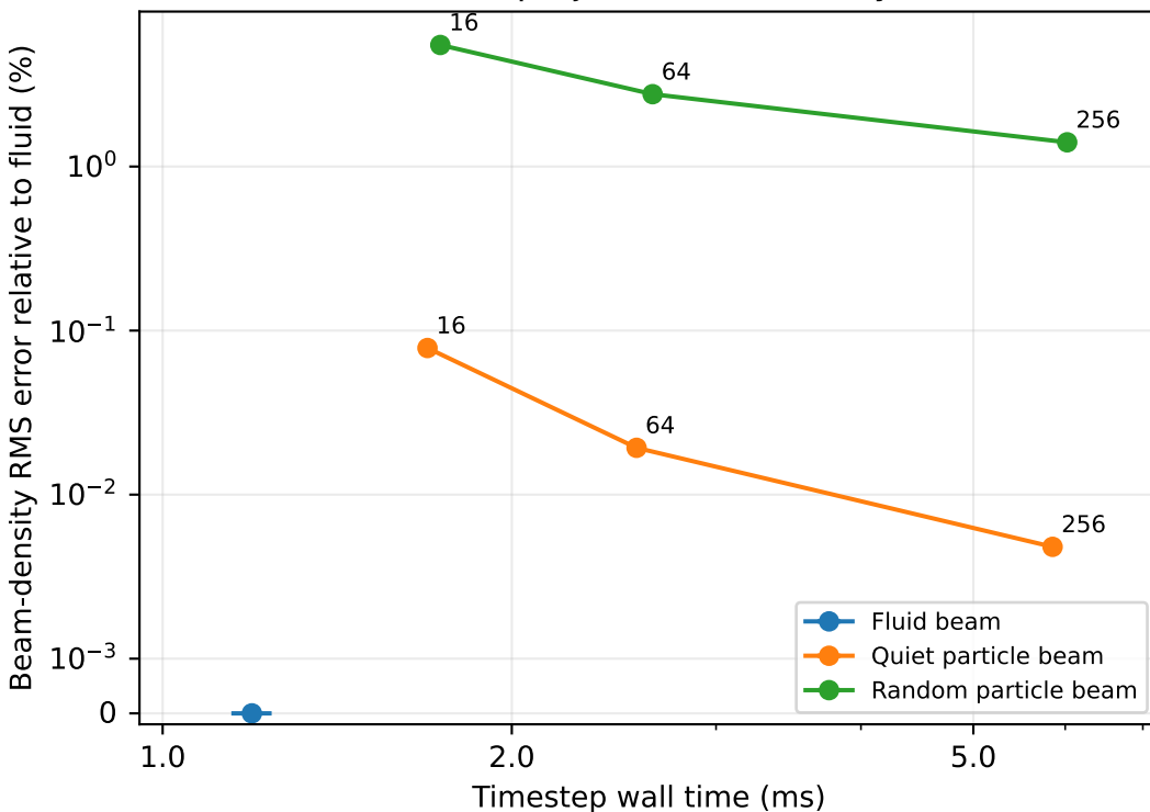
Beam projection: fields only
