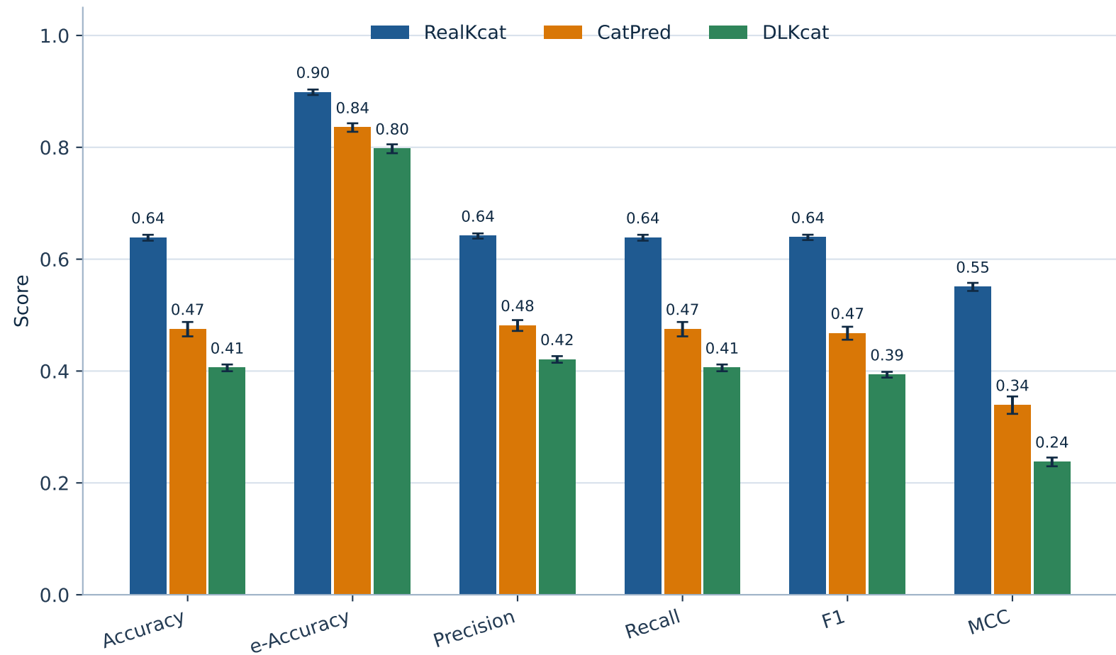
All-Fold Test Benchmark (mean \pm SD)
