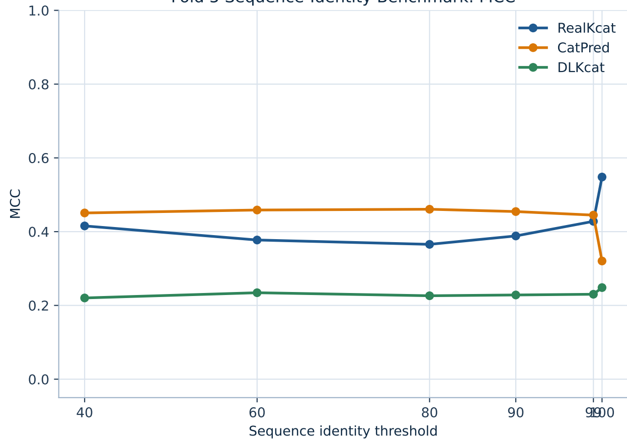
Fold 5 Sequence-Identity Benchmark: MCC
