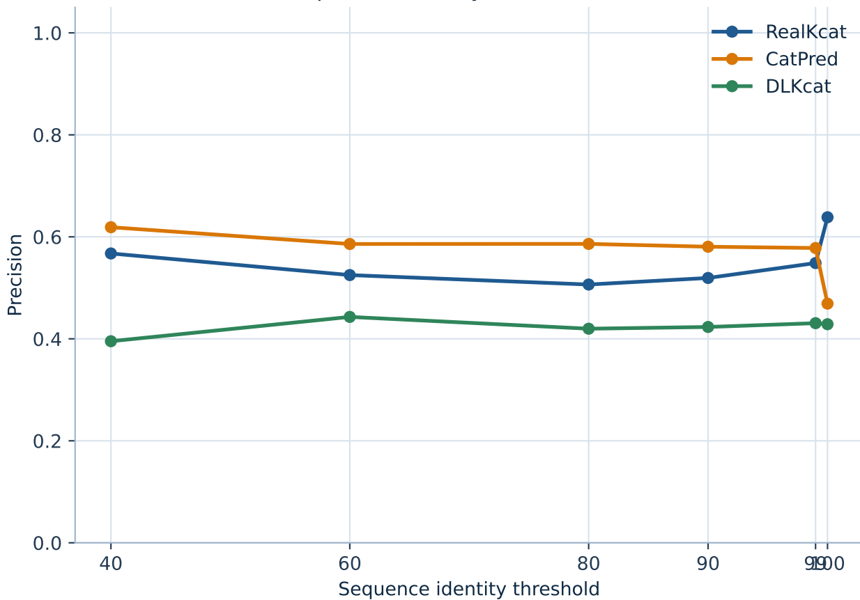
Fold 5 Sequence-Identity Benchmark: Precision
