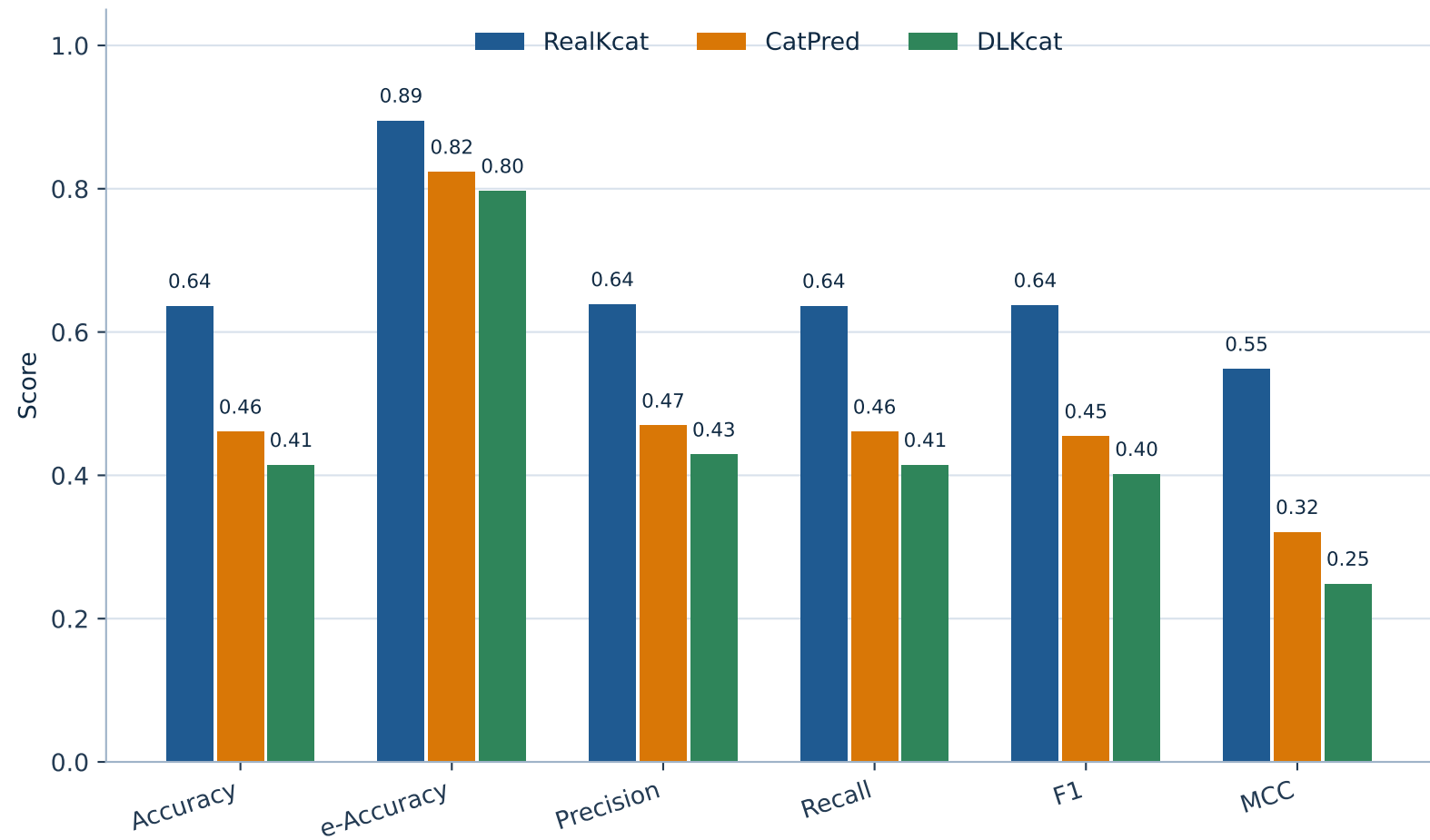
Fold 5 Test Benchmark
