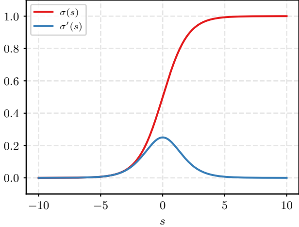
Sigmoid and its derivative
