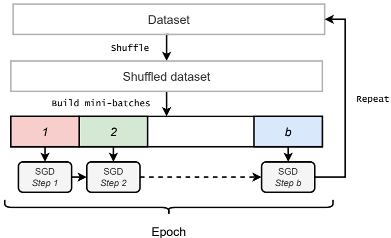
Figure 6: Dividing the optimization process into epochs is also helpful to define metrics and stopping criteria.
