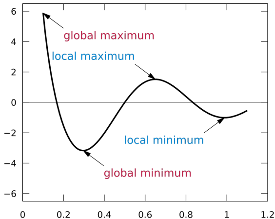
Figure 3: With no additional information, stationary points can be minima , maxima , and can be local or global (Wikimedia, KSmrq).
