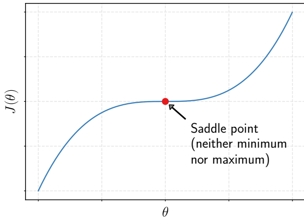
Figure 4: Stationary points can also be saddle points , either decreasing or increasing in different directions.
