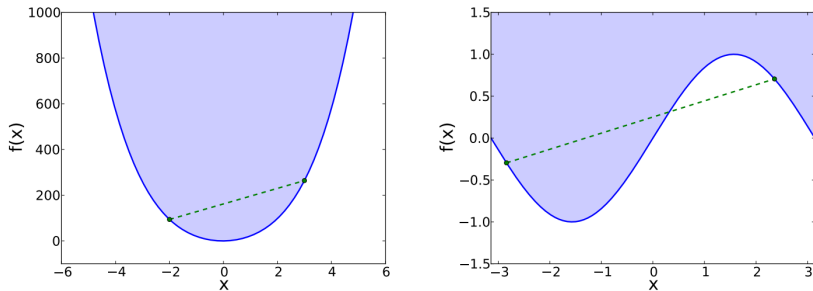
Figure 8: Left: an example of convex function. Right: an example of non-convex function. Taken from “An Introduction to Machine Learning” by Smola and Vishwanathan [unpublished].
