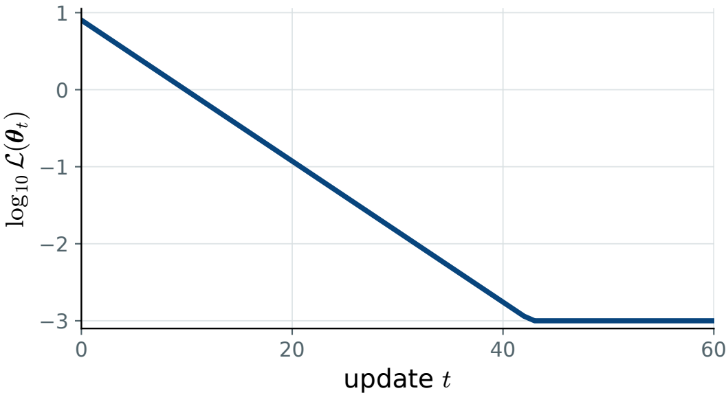
Full-batch GD
