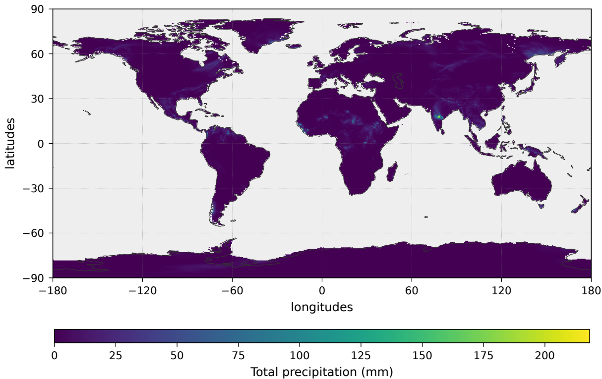
ERA5-Land total precipitation — 1 September 2024
