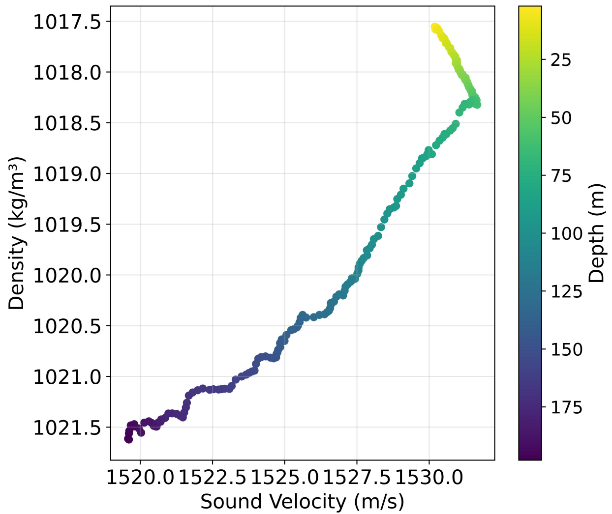
Figure 1.3: Sound speed and seawater density diagram from the SeaLabMOS CTD deployment. The same data as in Fig. 1.1.
