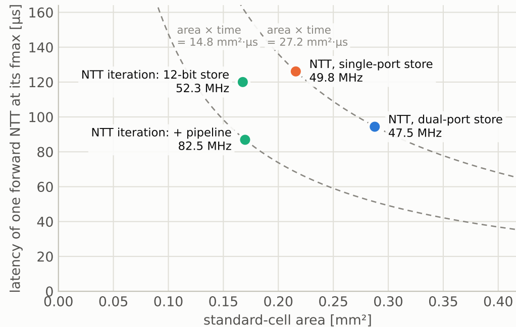
(a) NTT
