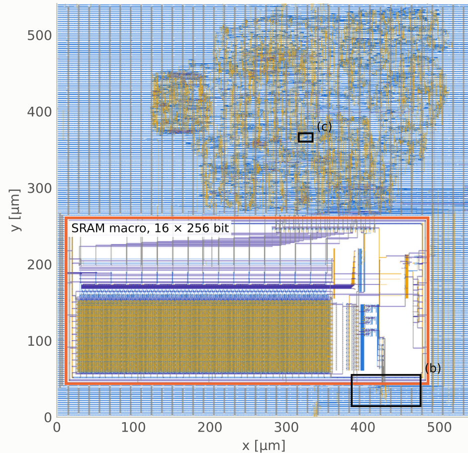
(a) Whole block, 541 \mu\text{m} square, metal 1-4
