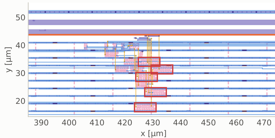
(b) Bottom edge of the macro: address-pin drivers (red) at the halo
