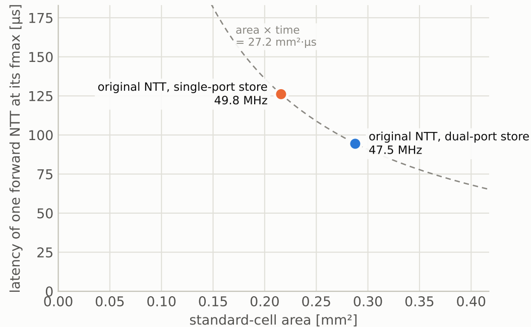
(a) NTT
