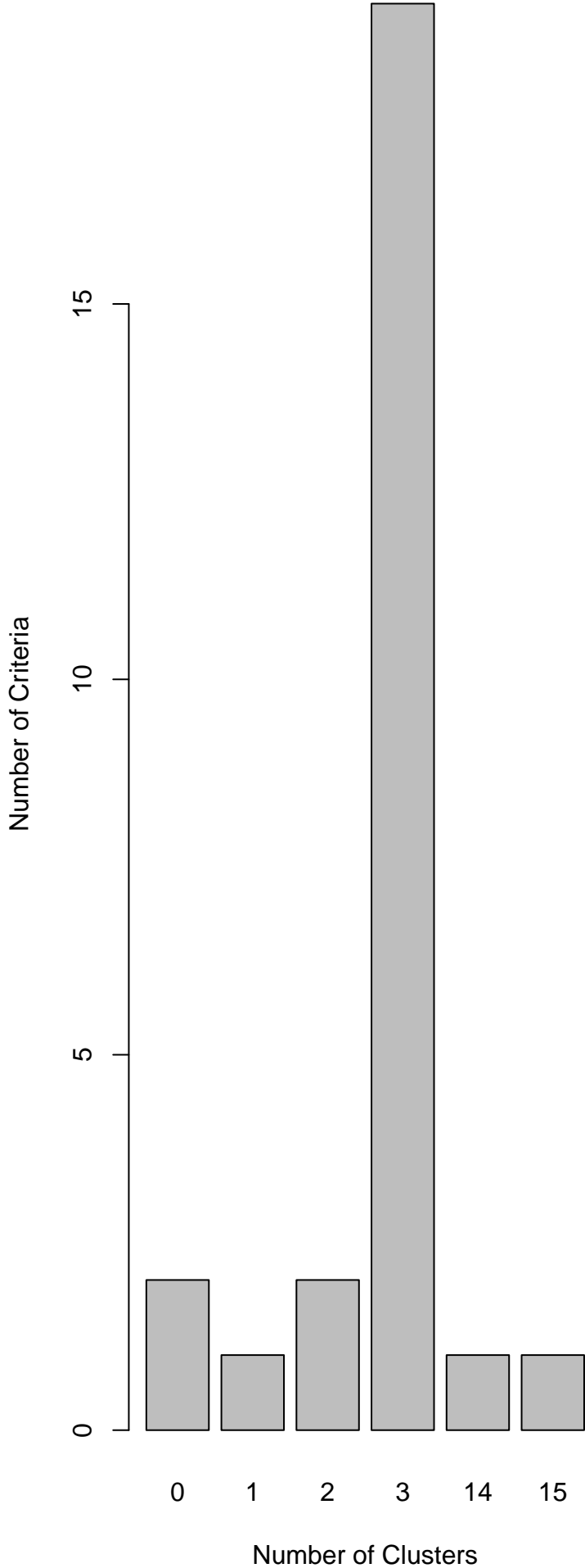
Number of Clusters Chosen by 26 Criteria
