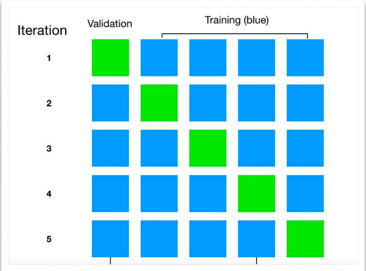
cross-validation
