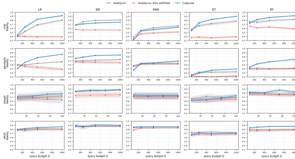
Figure 2: Fidelity vs. query budget for Autolyucus (grey, dashed), Autolyucus with bin edges withheld (red, dotted) and CUTPURSE (blue, solid), per dataset (rows) and target (columns), for the four datasets with continuous features. Band is the standard error over ten independent target instantiations. Same splits, seed sets and attack RNG as Table 6, whose cells are the rightmost point of each curve.
