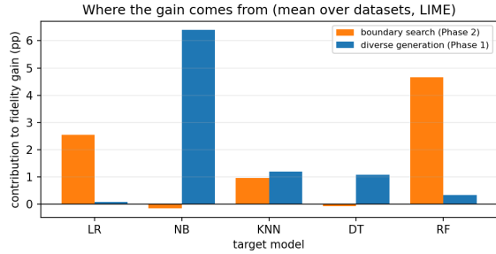
Figure 3: Contribution of each component to the LIME fidelity gain over Autolytus (percentage points, mean over datasets, top budget). Boundary search dominates for RF/LR; diverse generation dominates for NB.
