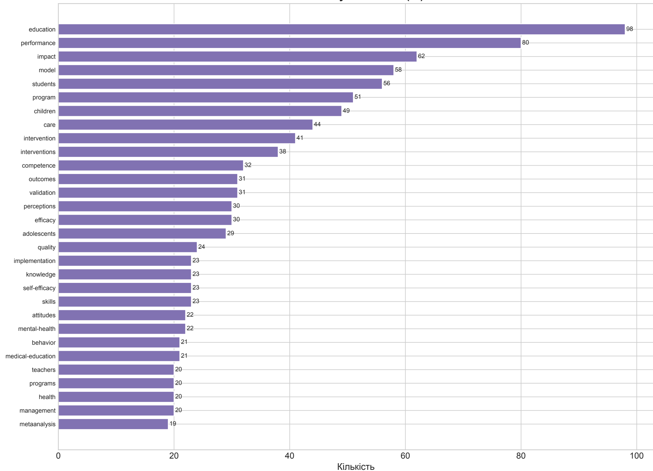
Ton-30 Keywords Plus (ID)
