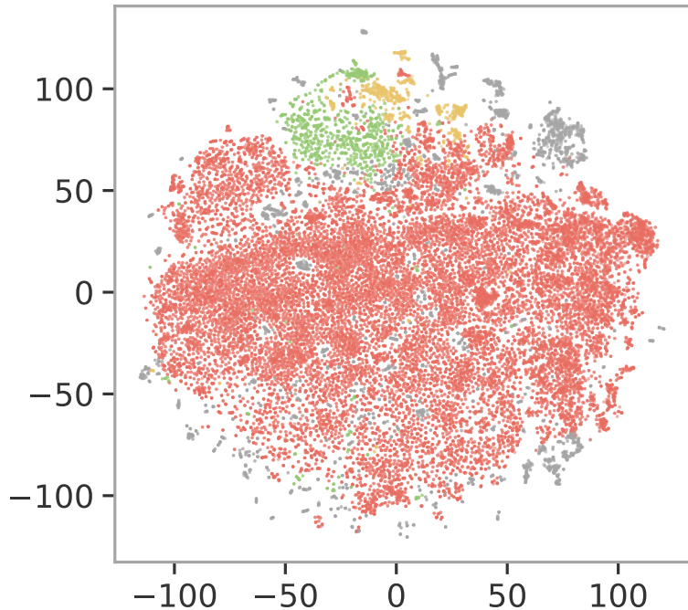
Drosophila spp. - t-SNE
