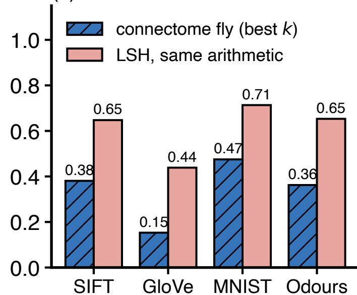
(c) MaleCNS connectome
