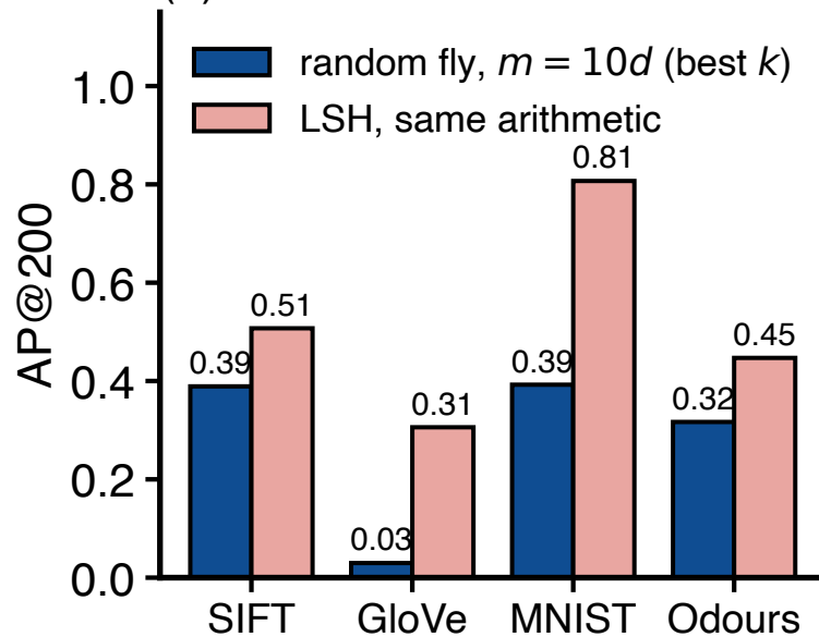
(b) random matrices
