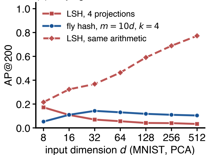
(a) varying d , one dataset
