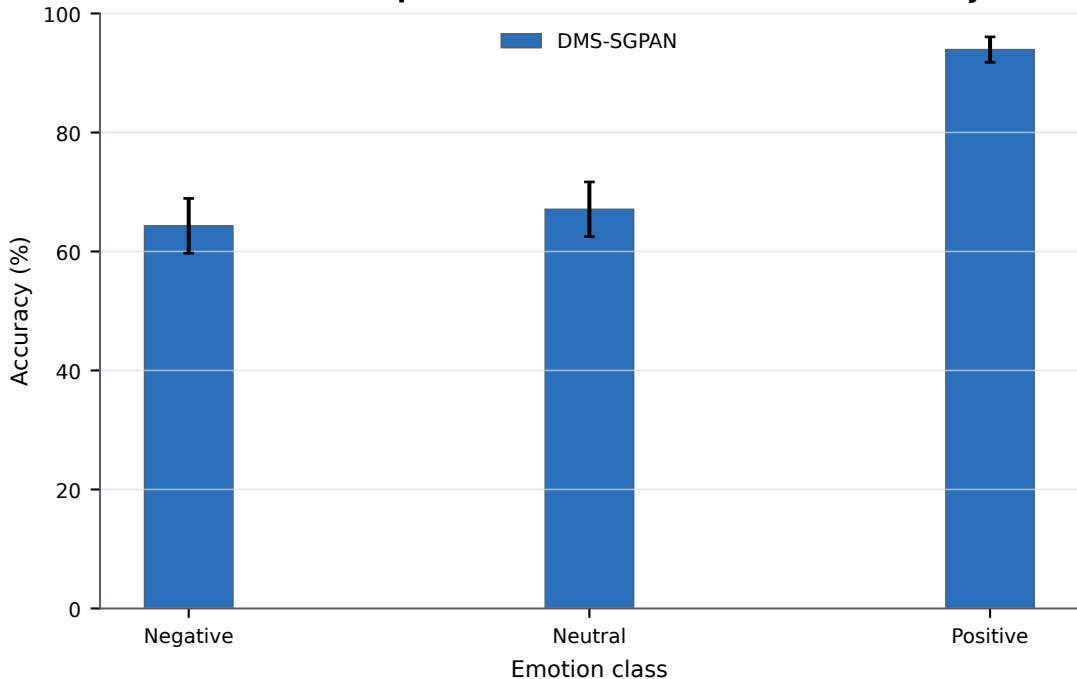
SEED: class-wise performance on held-out TVT test subjects
