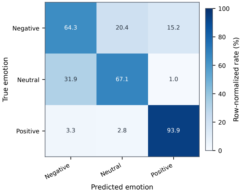
SEED: DMS-SGPAN confusion matrix
